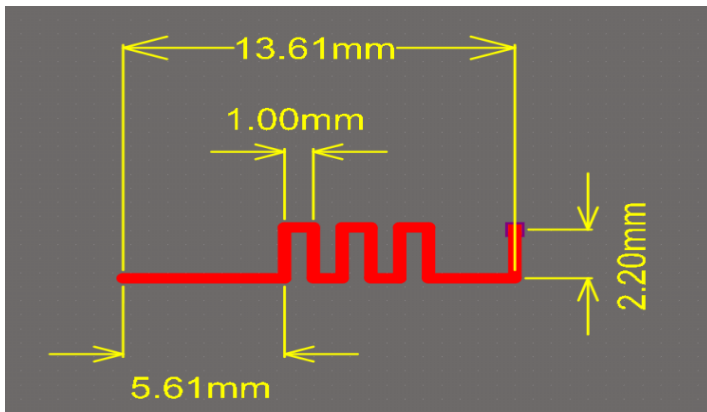
Antenna Photo & Length ( mm )
