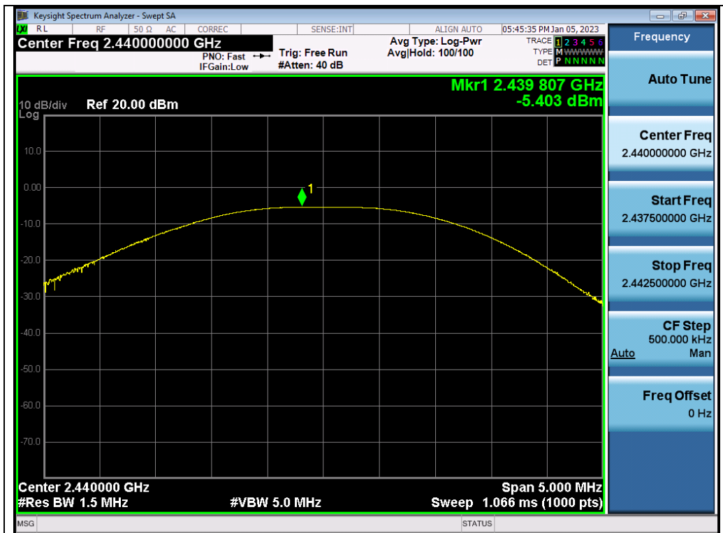
Test_Graph_BLE1M_ANT1_2440_1Mbps_Peak Power
