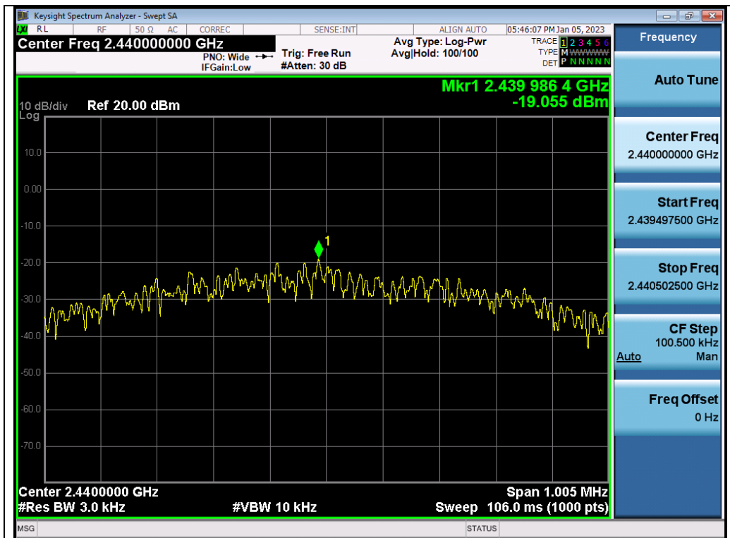
Test_Graph_BLE1M_ANT1_2440_1Mbps_PSD
