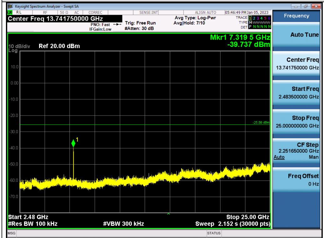
Test_Graph_BLE1M_ANT1_2440_1Mbps_Higher Band Emissions
