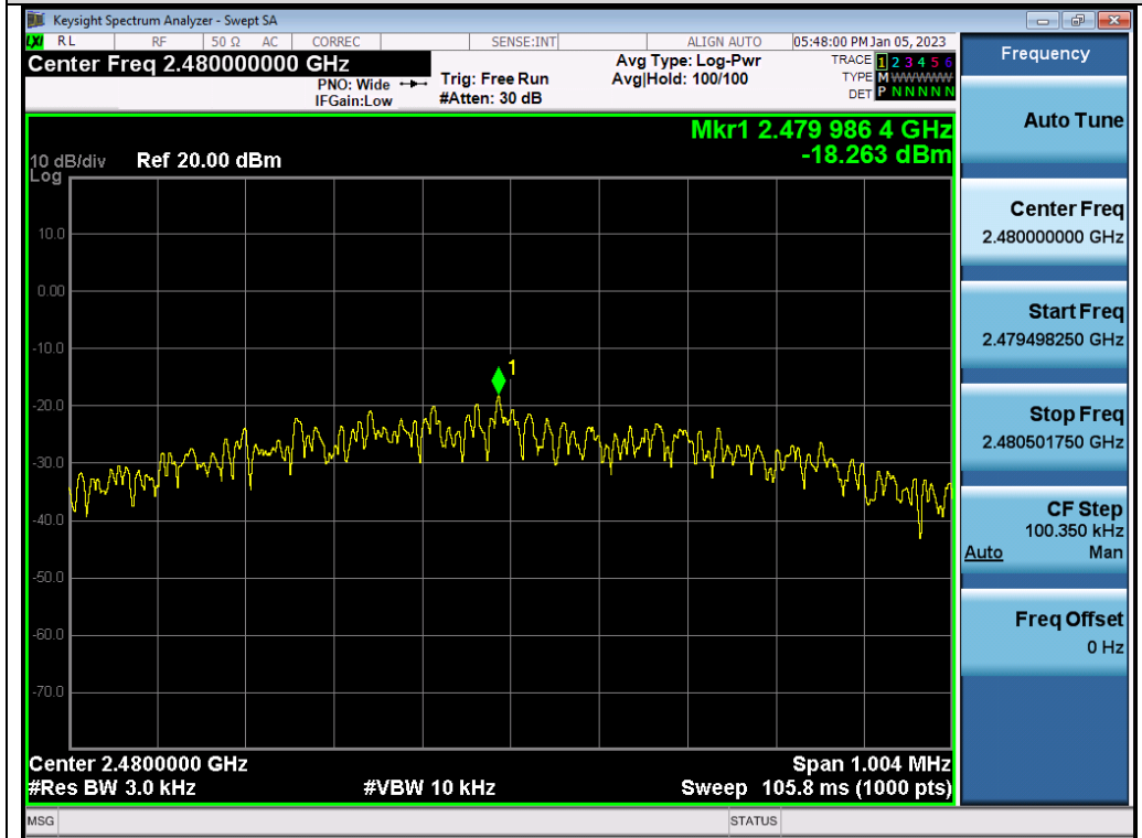
Test_Graph_BLE1M_ANT1_2480_1Mbps_PSD
