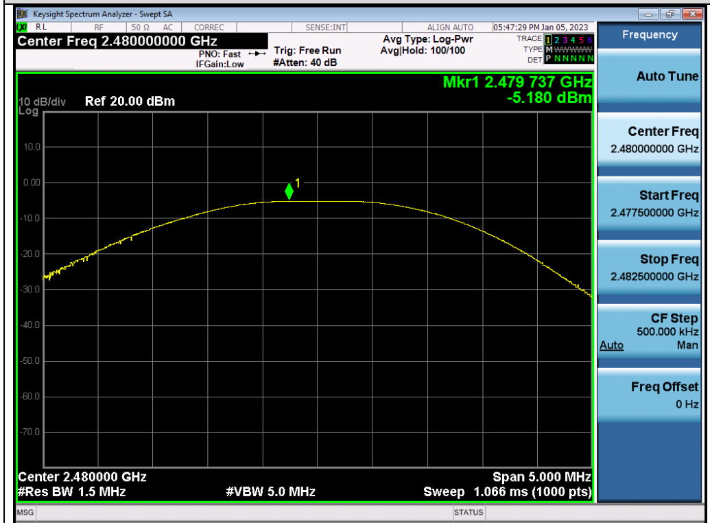
Test_Graph_BLE1M_ANT1_2480_1Mbps_Peak Power
