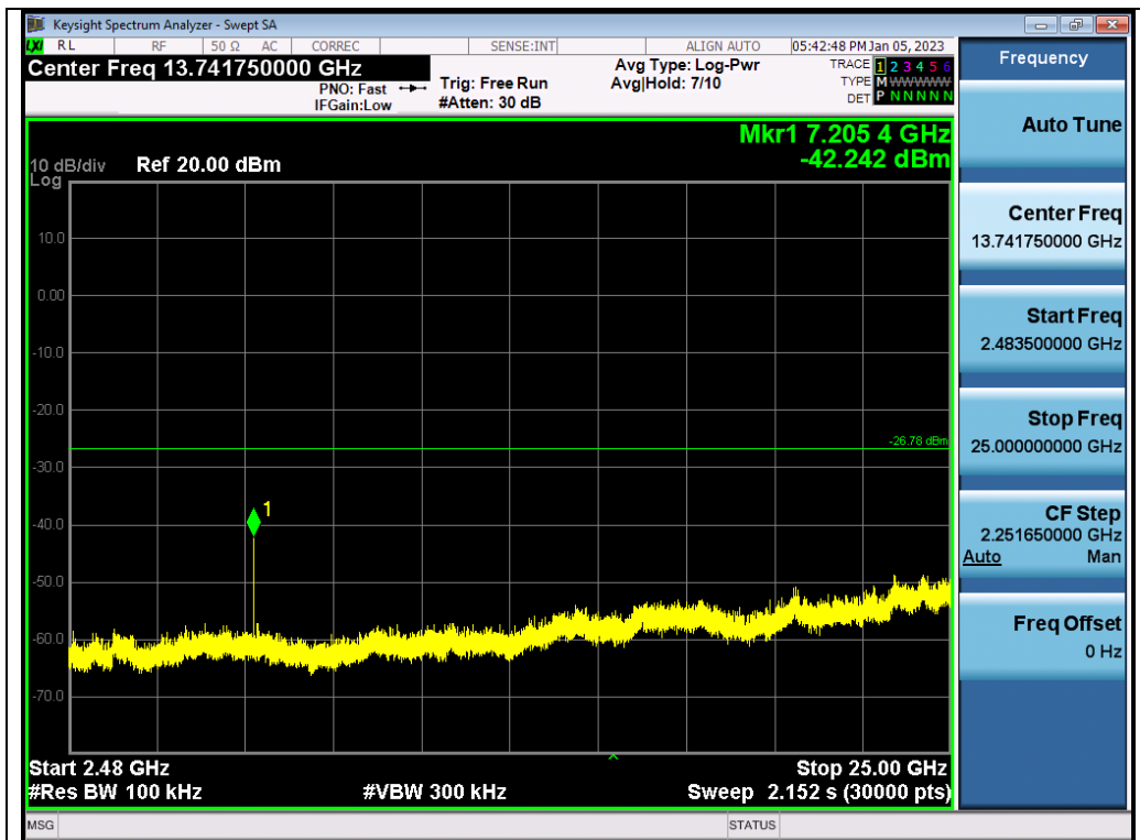
Test_Graph_BLE1M_ANT1_2402_1Mbps_Higher Band Emissions
