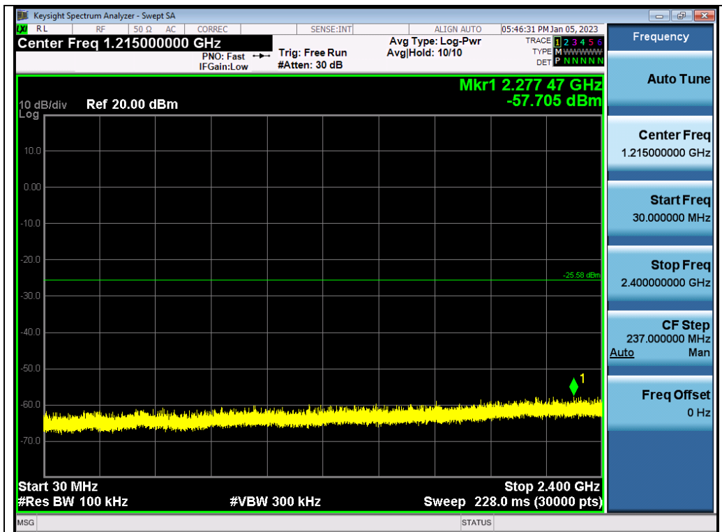
Test_Graph_BLE1M_ANT1_2440_1Mbps_Lower Band Emissions
