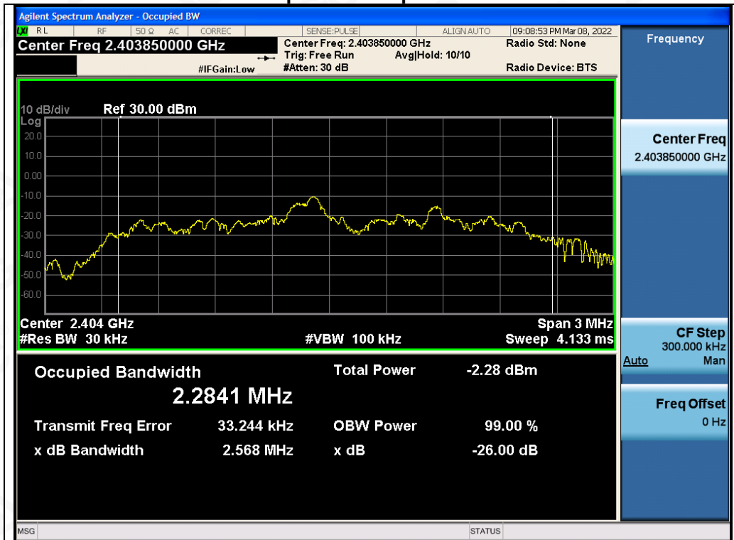
Test_Graph_LE1M_ANT1_2403.85_1Mbps_OBW
