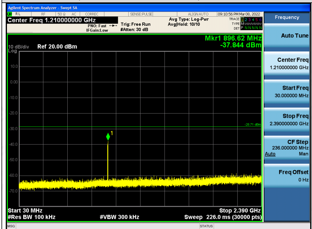
Test_Graph_LE1M_ANT1_2403.85_1Mbps_Lower Band Emissions
