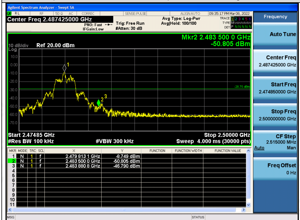
Test_Graph_LE1M_ANT1_2479.85_1Mbps_Higher Band Edge Emissions
