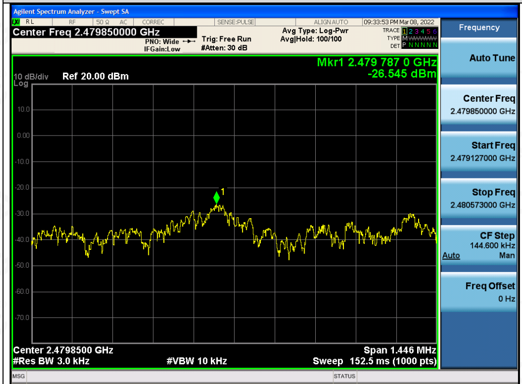
Test_Graph_LE1M_ANT1_2479.85_1Mbps_PSD
