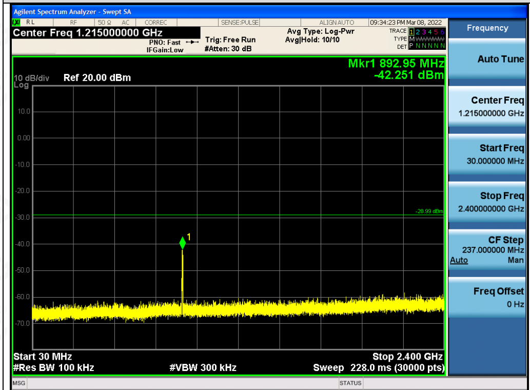
Test_Graph_LE1M_ANT1_2479.85_1Mbps_Lower Band Emissions
