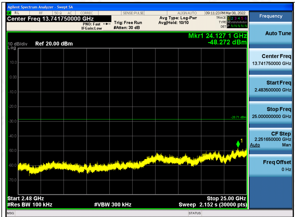
Test_Graph_LE1M_ANT1_2403.85_1Mbps_Higher Band Emissions
