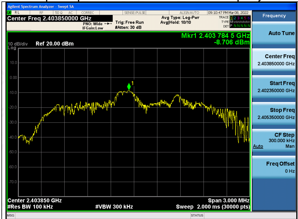
Test_Graph_LE1M_ANT1_2403.85_1Mbps_Reference Level
