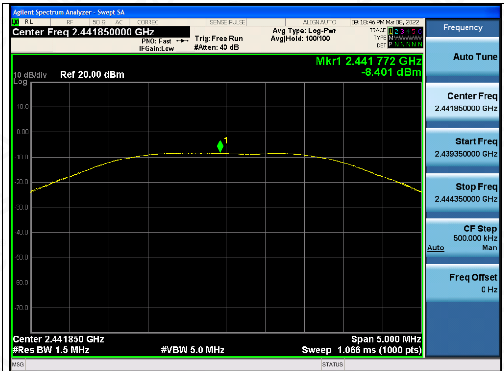
Test_Graph_LE1M_ANT1_2441.85_1Mbps_Peak Power
