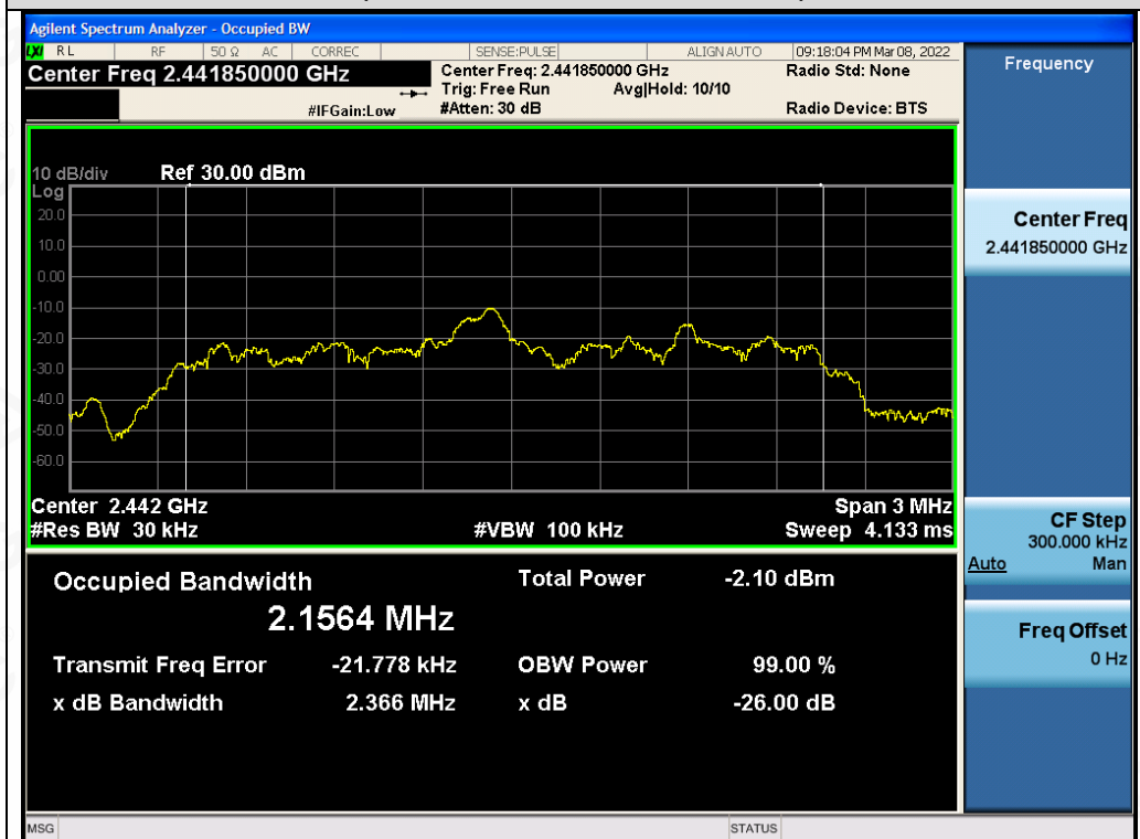
Test_Graph_LE1M_ANT1_2441.85_1Mbps_OBW
