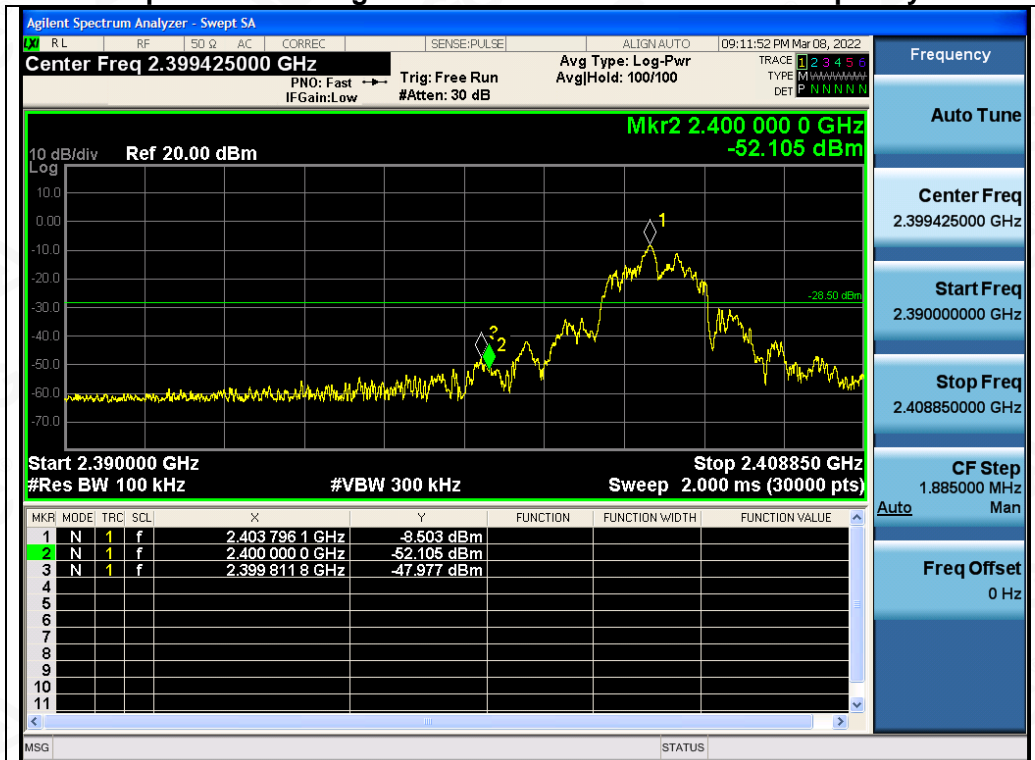
Test_Graph_LE1M_ANT1_2403.85_1Mbps_Lower Band Edge Emissions
