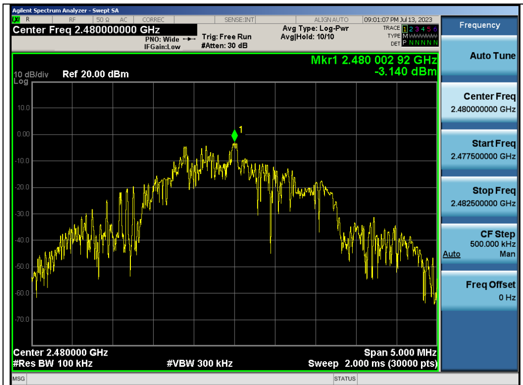
Test_Graph_2.4G_ANT1_2480_2Mbps_Reference Level
