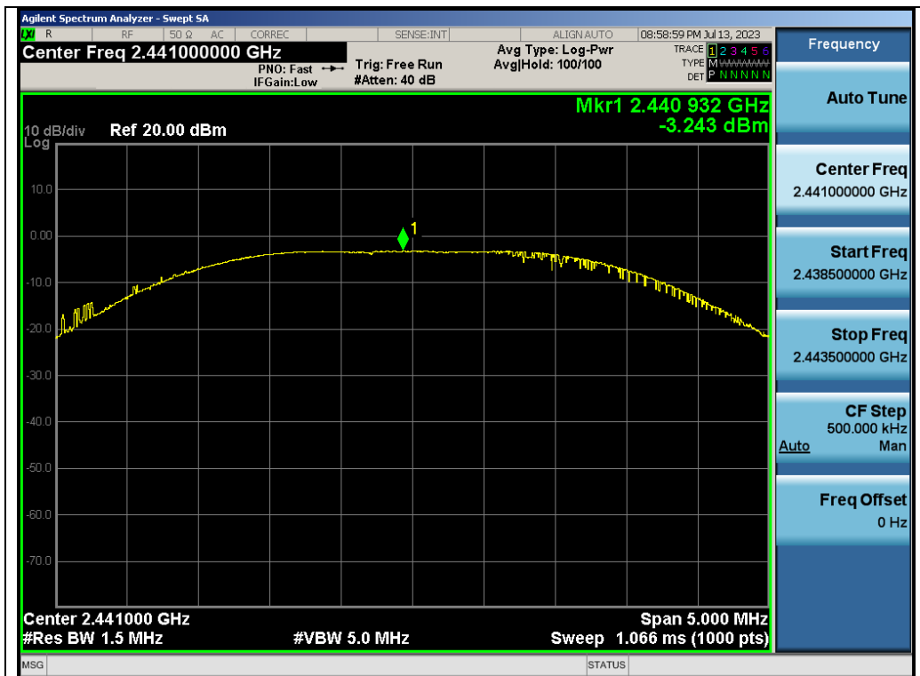
Test_Graph_2.4G_ANT1_2441_2Mbps_Peak Power
