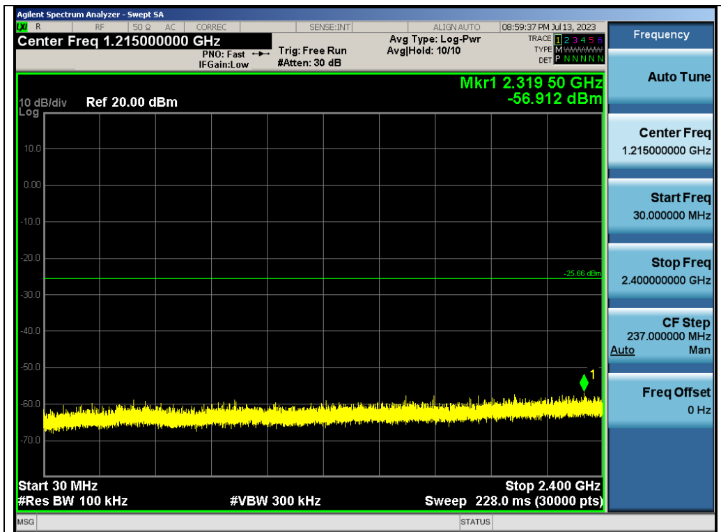
Test_Graph_2.4G_ANT1_2441_2Mbps_Lower Band Emissions
