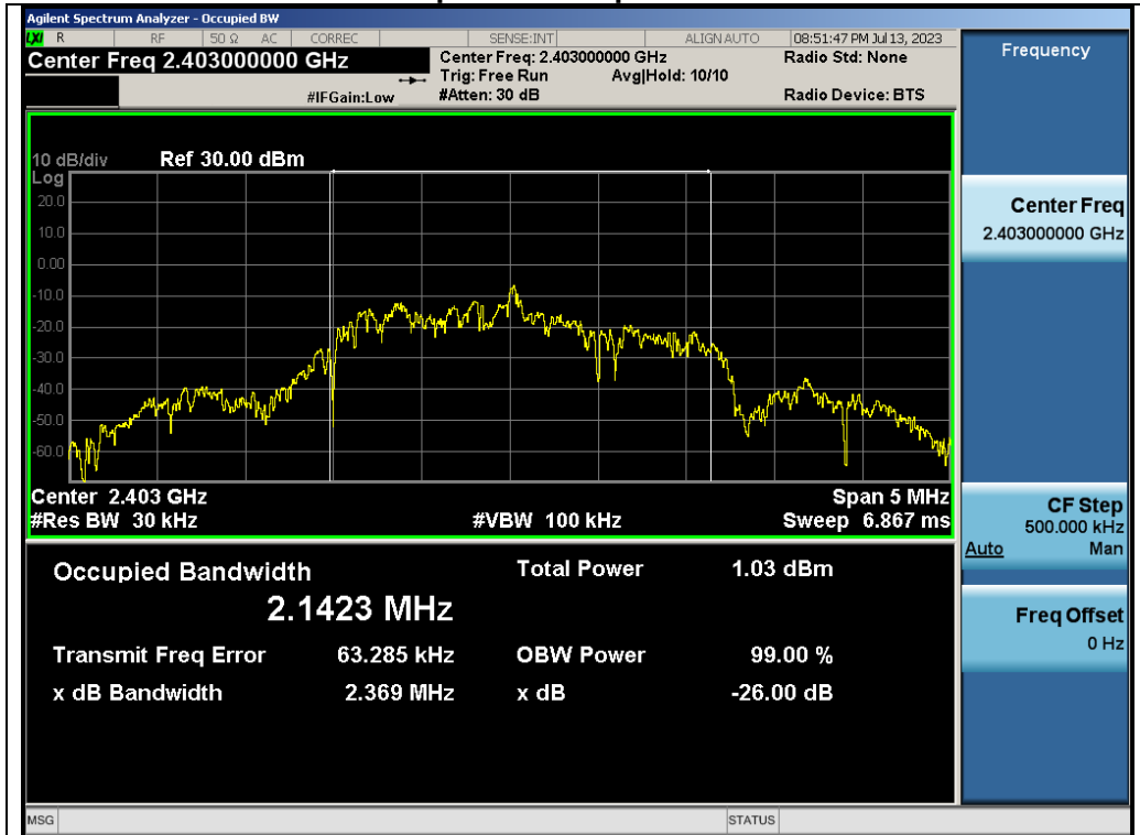
Test_Graph_2.4G_ANT1_2403_2Mbps_OBW
