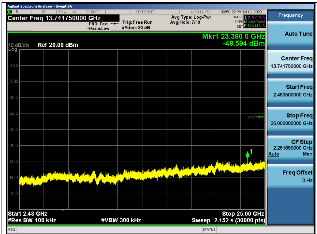
Test_Graph_2.4G_ANT1_2403_2Mbps_Higher Band Emissions
