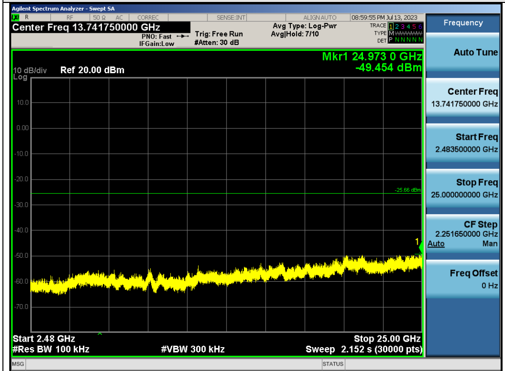
Test_Graph_2.4G_ANT1_2441_2Mbps_Higher Band Emissions
