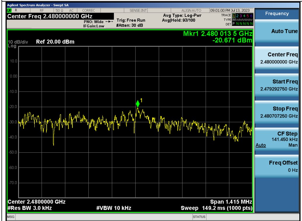
Test_Graph_2.4G_ANT1_2480_2Mbps_PSD
