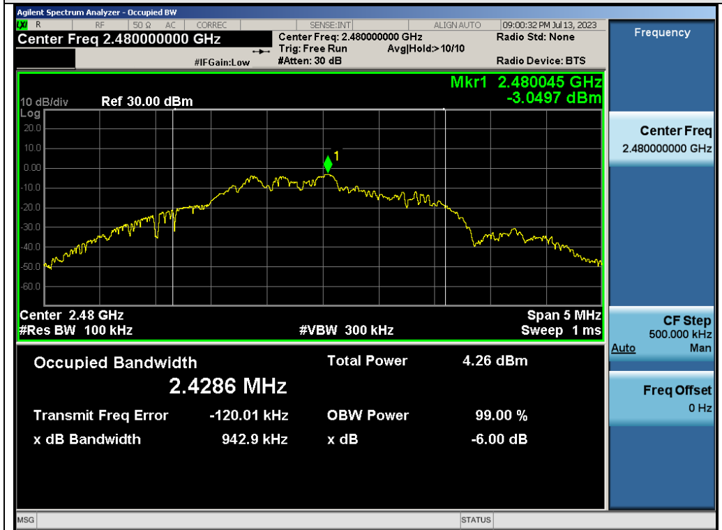
Test_Graph_2.4G_ANT1_2480_2Mbps_DTSBW
