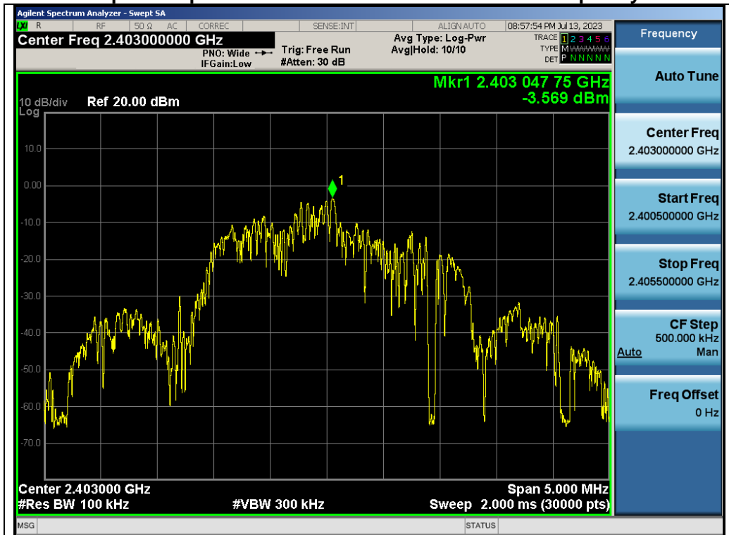
Test_Graph_2.4G_ANT1_2403_2Mbps_Reference Level
