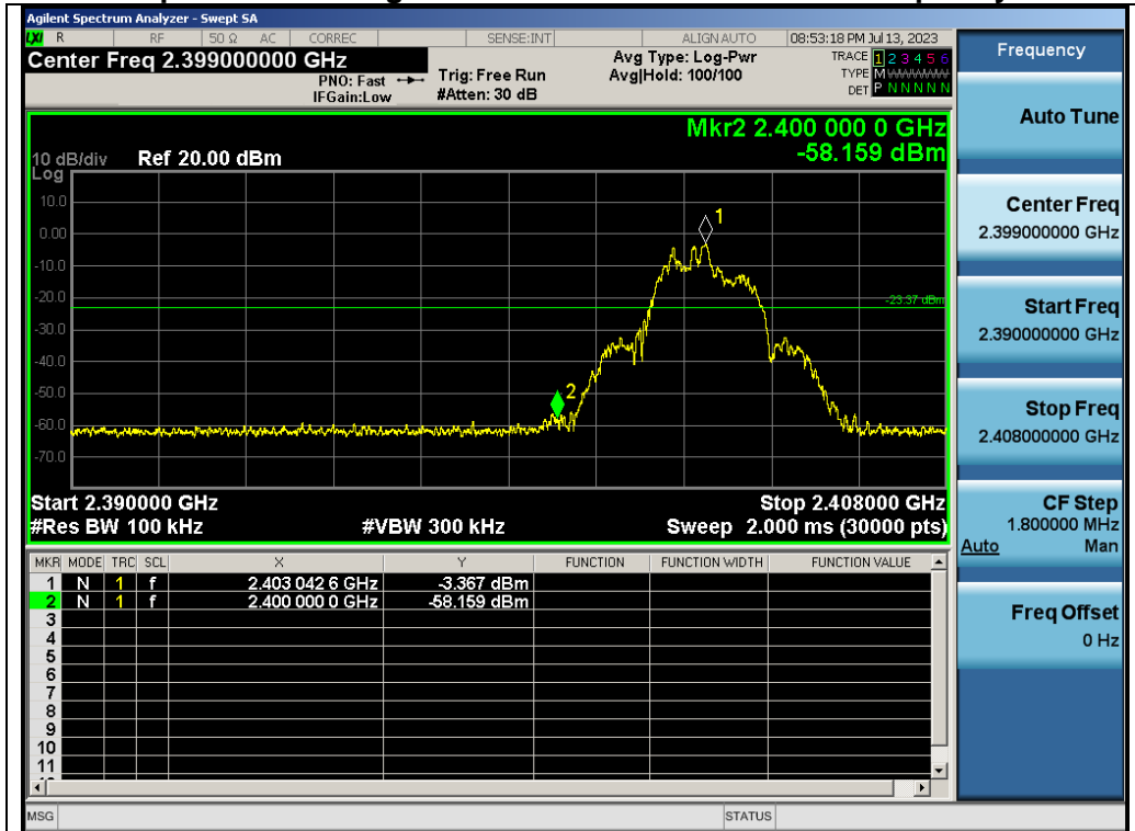
Test_Graph_2.4G_ANT1_2403_2Mbps_Lower Band Edge Emissions
