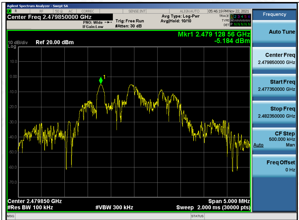
Test_Graph_ANT1_2479.85_Reference Level
