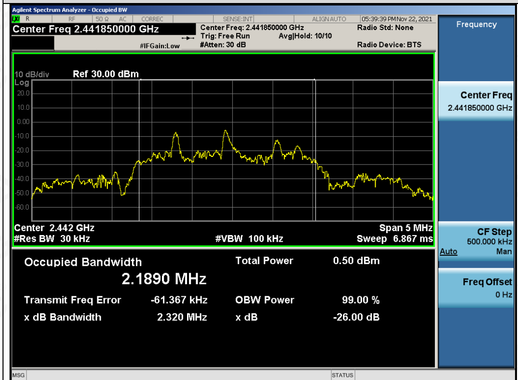
Test_Graph_ANT1_2441.85_OBW
