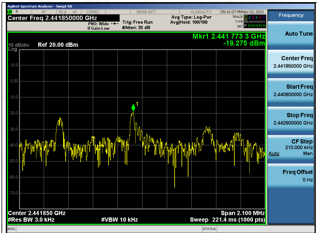
Test_Graph_LE2M_ANT1_2441.85_2Mbps_PSD
