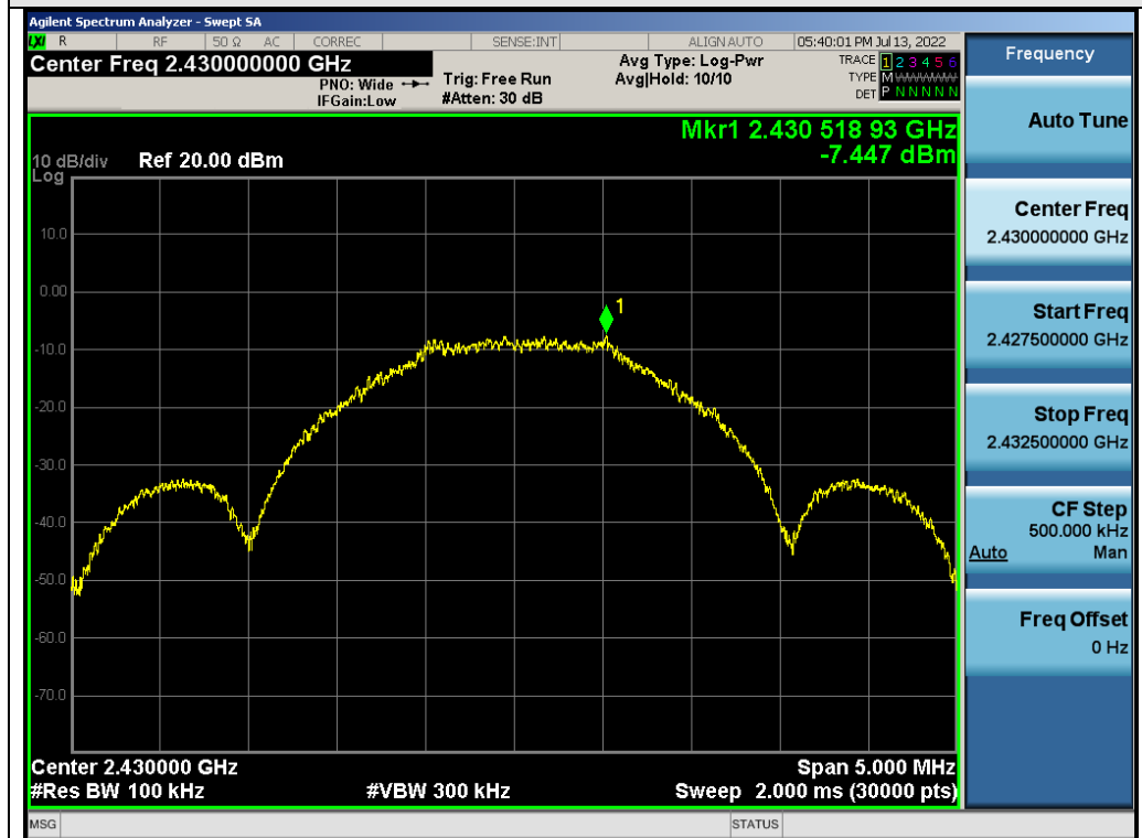
Test_Graph_2.4G_ANT1_2430_Reference Level
