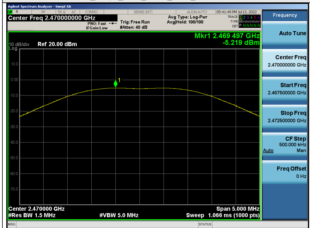
Test_Graph_2.4G_ANT1_2470_Peak Power
