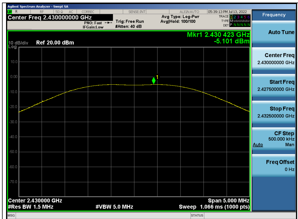
Test_Graph_2.4G_ANT1_2430_Peak Power
