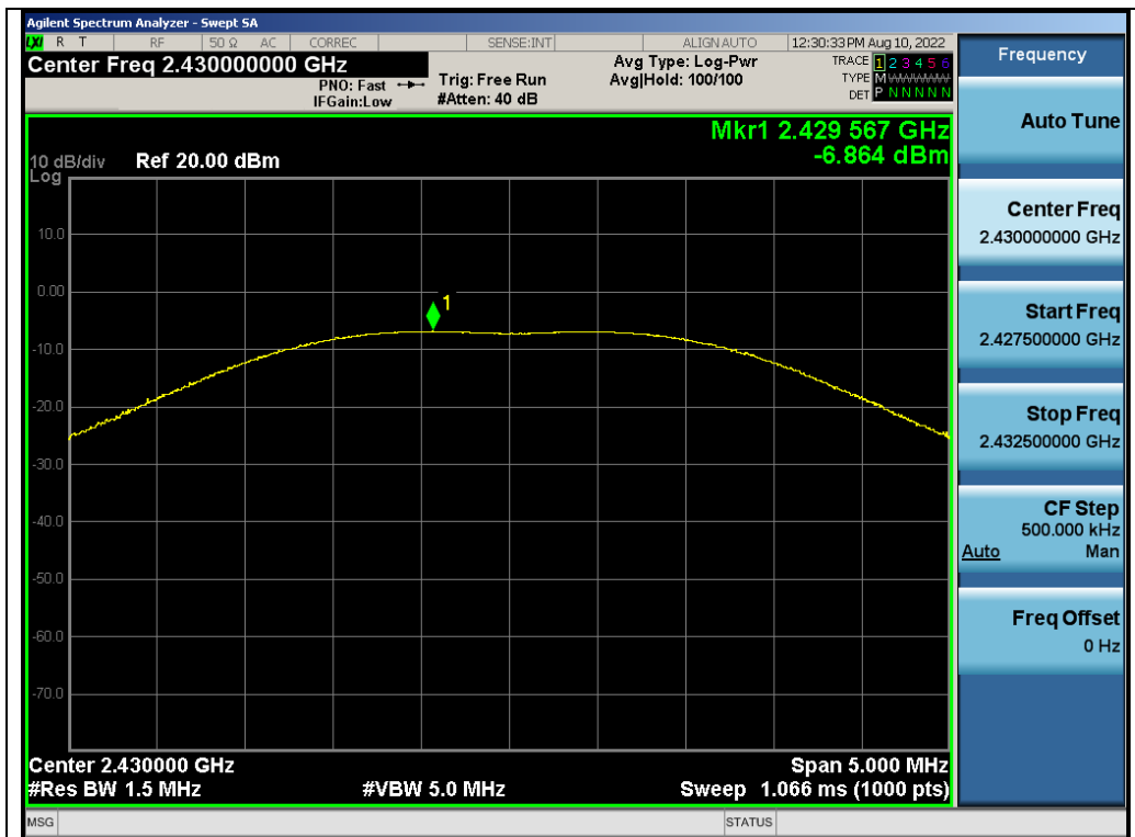
Test_Graph_GFSK_ANT1_2430_Peak Power
