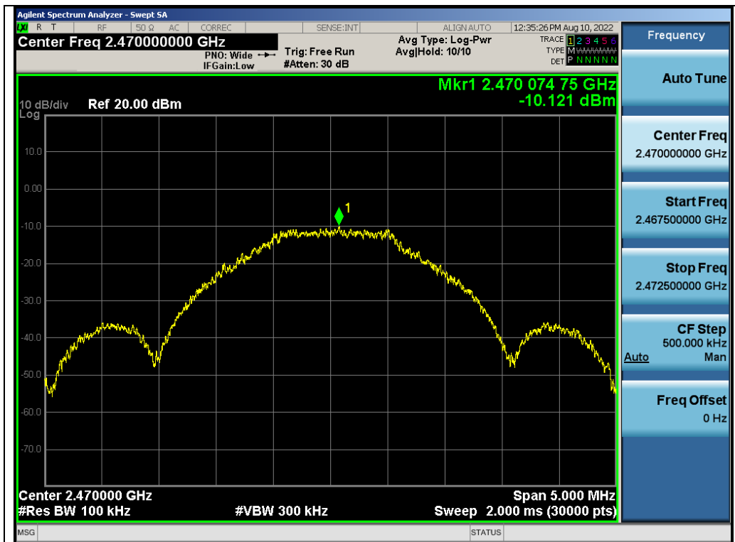
Test_Graph_GFSK_ANT1_2470_Reference Level
