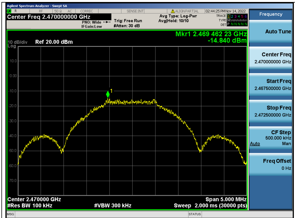
Test_Graph_GFSK_ANT1_2470_Reference Level
