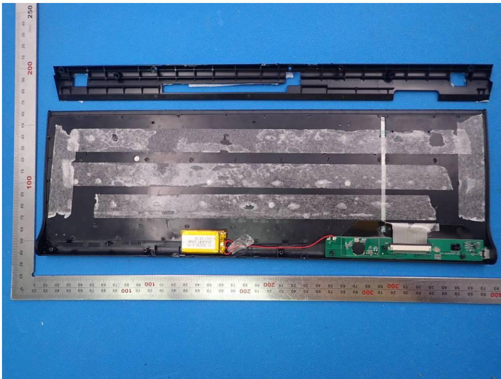
INTERNAL VIEW OF EUT-1(HW193)
