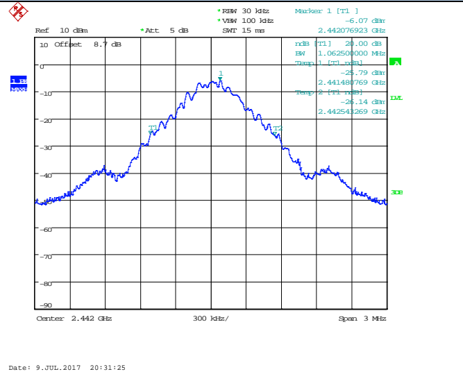
Channel 7 / 2442 MHz
