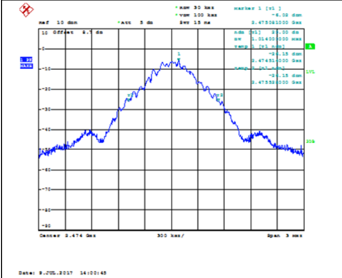
Channel 12 / 2474 MHz
