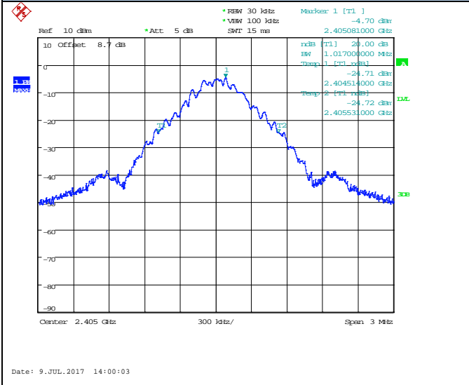
Channel 1 / 2405 MHz
