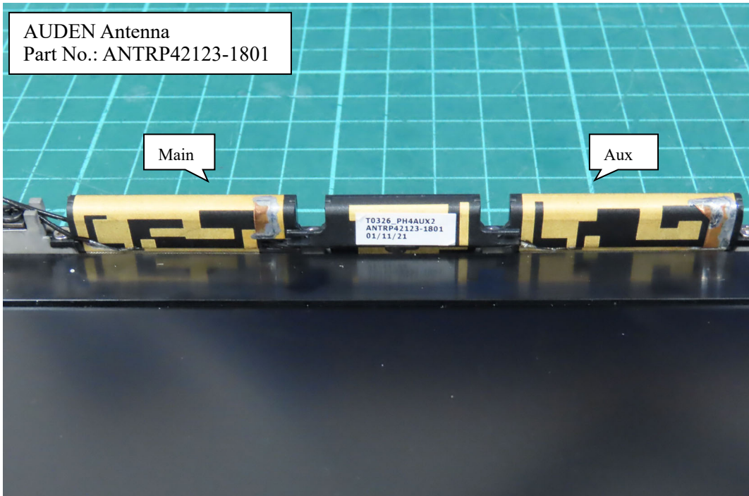
(22) EUT Photo
