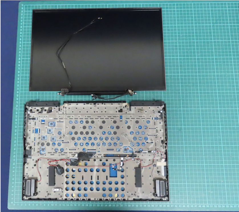
(25) EUT Photo
