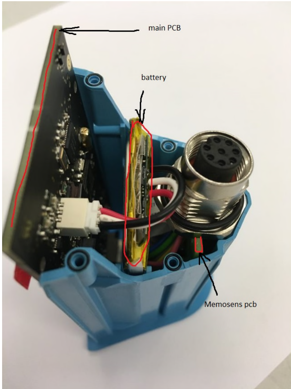
View without the outer enclosure Position of the two pcb and the battery
