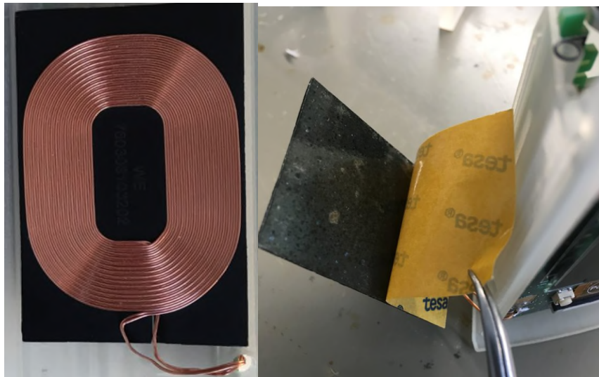
Qi charging coil front and rear side
