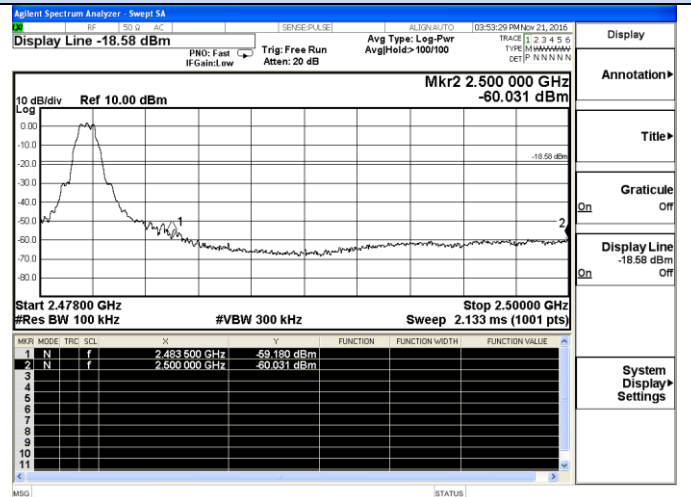
Channel 39 / 2480 MHz
