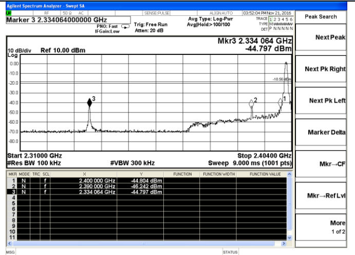
Channel 0 / 2402 MHz
