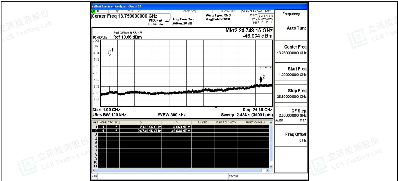
11N20SISO_Ant1_2437_0~Reference
