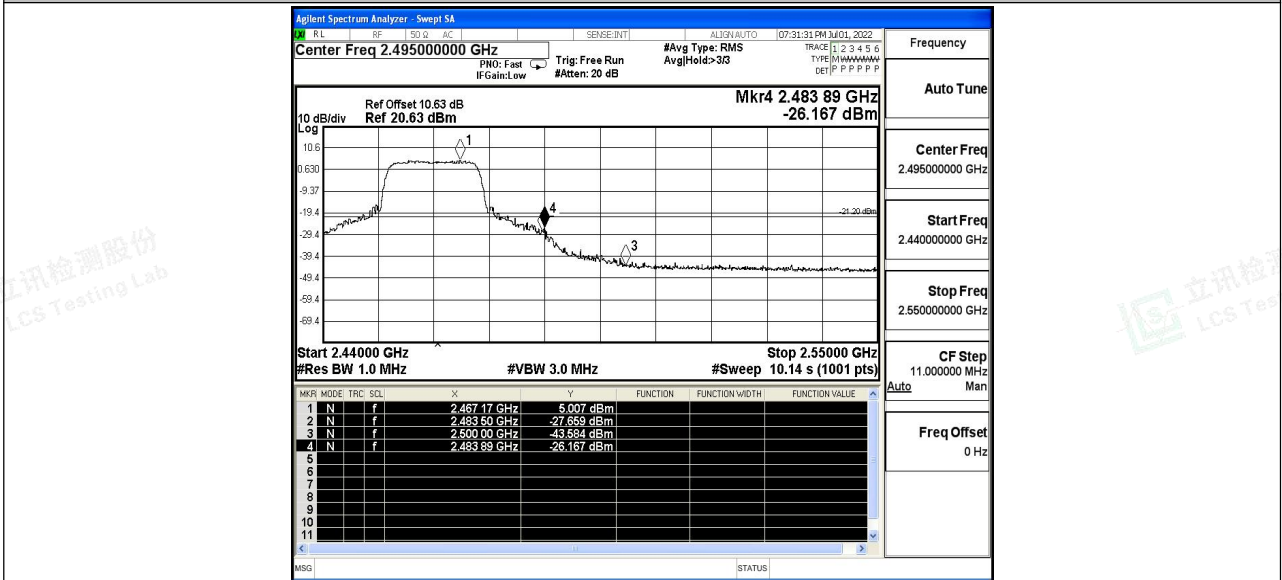
11N20SISO_Ant1_High_2462_Peak
