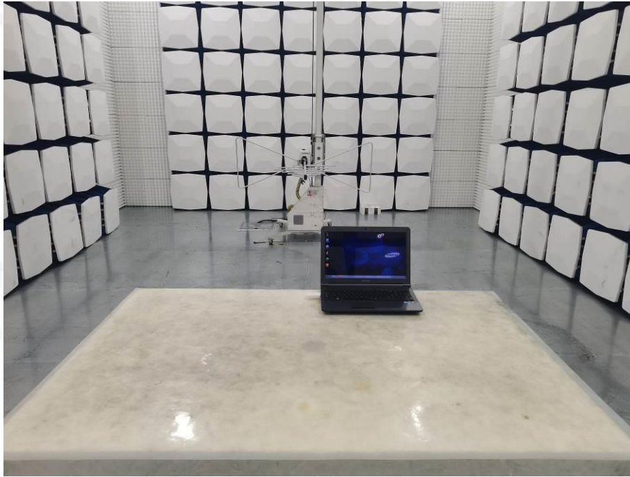
EUT Test Setup photo
