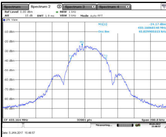
Figure 7.4.2-3: 99% Bandwidth – LCH
