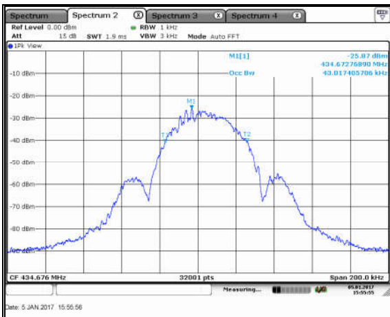
Figure 7.4.2-4: 99% Bandwidth – HCH
