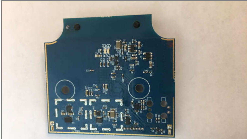
Figure 3: Internal Photo
