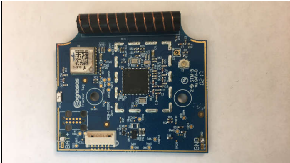
Figure 2: Internal Photo
