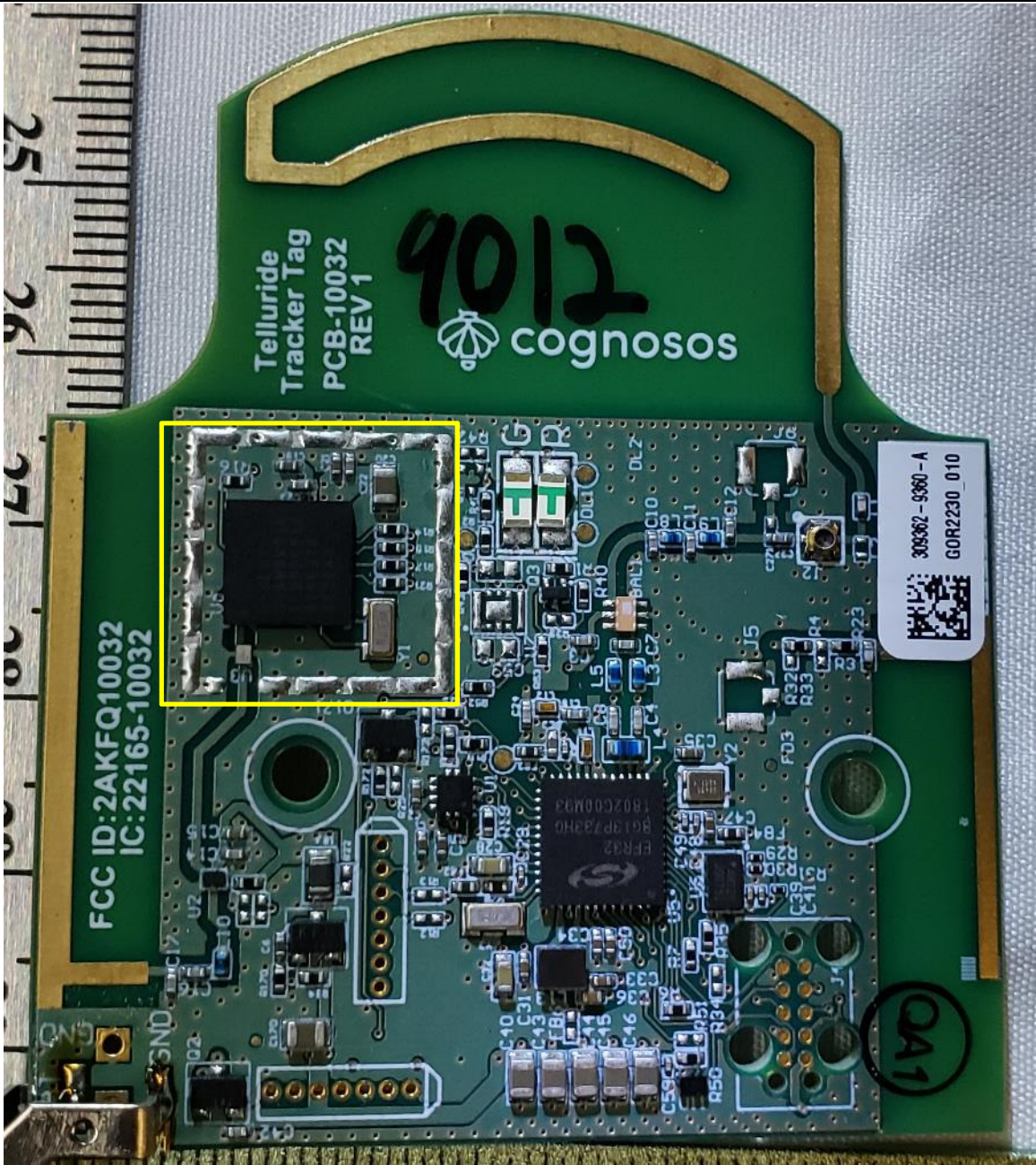
Figure 3. Radio Circuit
