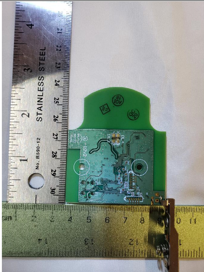
Figure 2. PCB – Back
