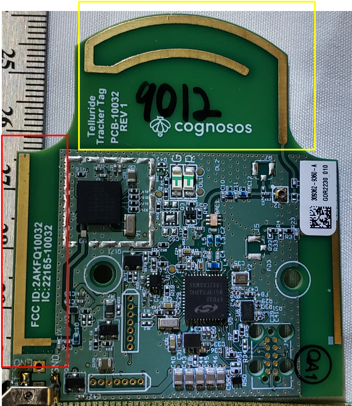
Figure 1. Radio Circuit
