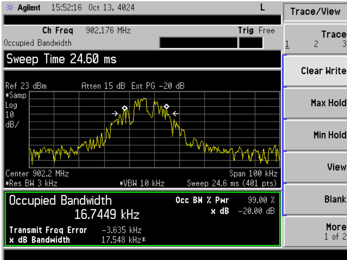
Figure 10. Bandwidth – Low Channel
