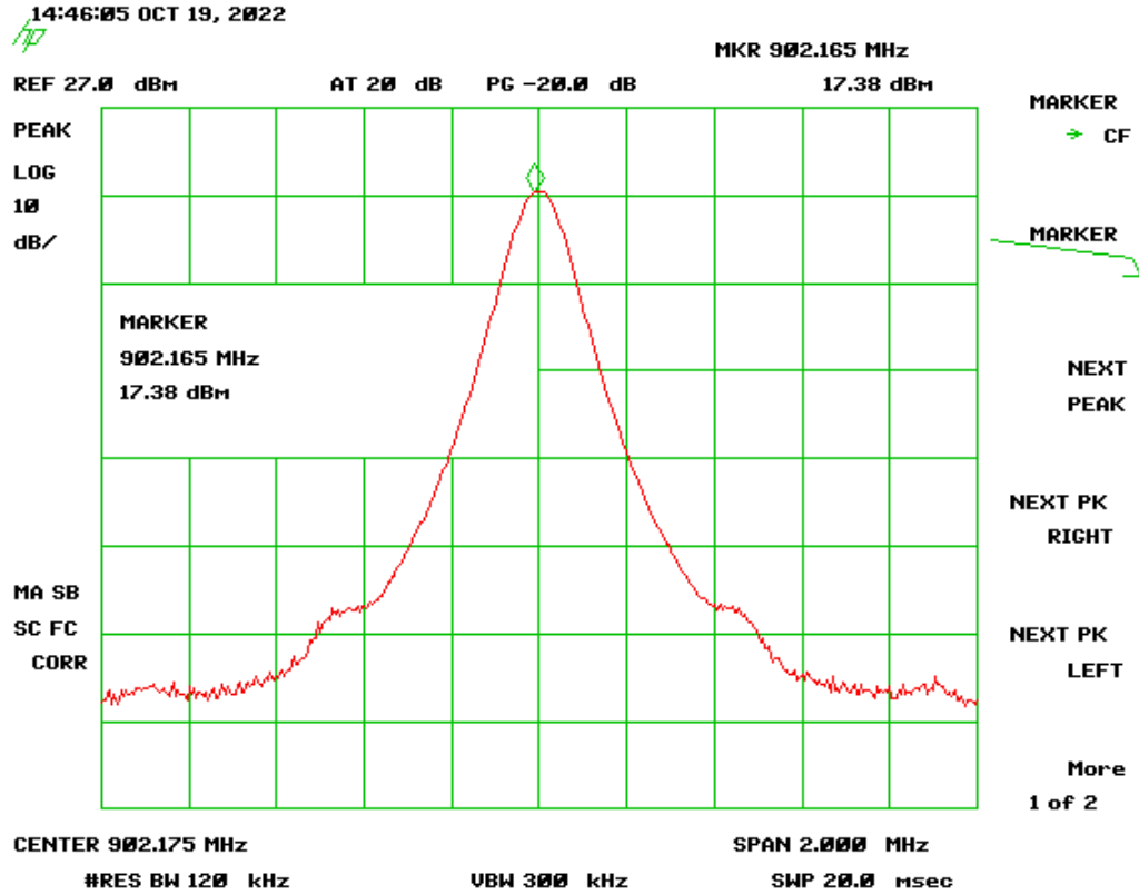
Figure 14. Peak Antenna Conducted Output Power, Low Channel
