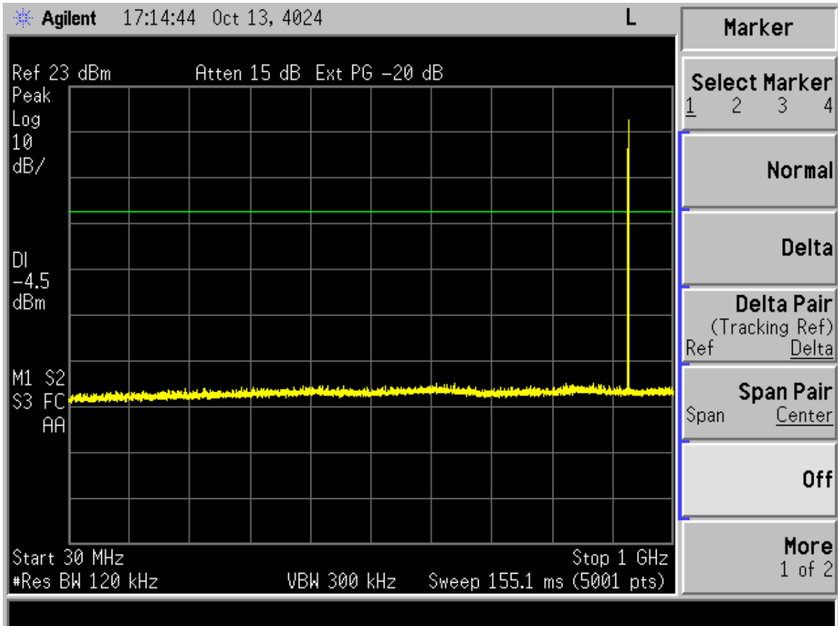
Figure 6. Conducted Spurious Emissions - High Channel, 30 MHz – 1 GHz
