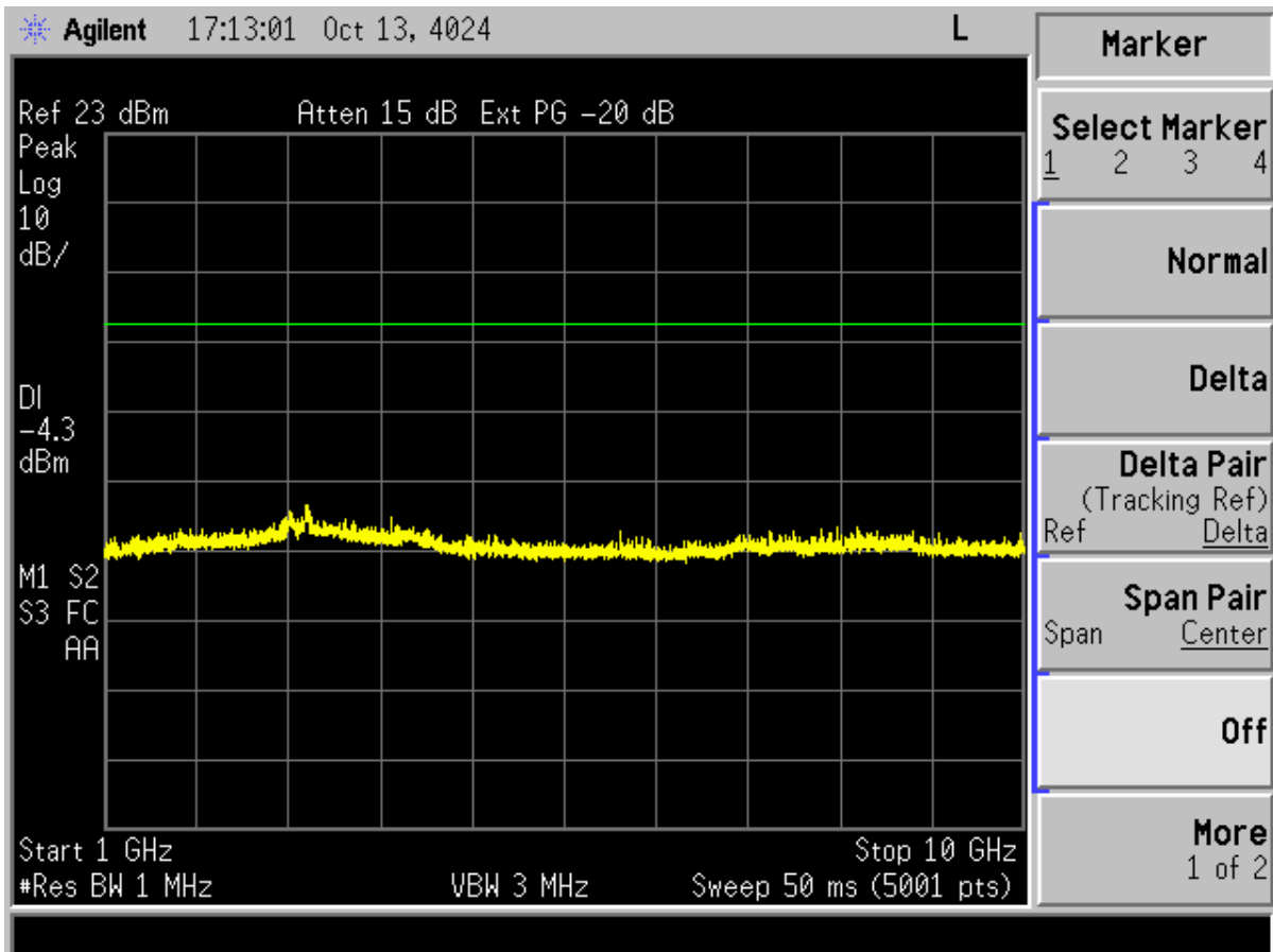
Figure 5. Conducted Spurious Emissions - Mid Channel, 1 GHz – 10 GHz
