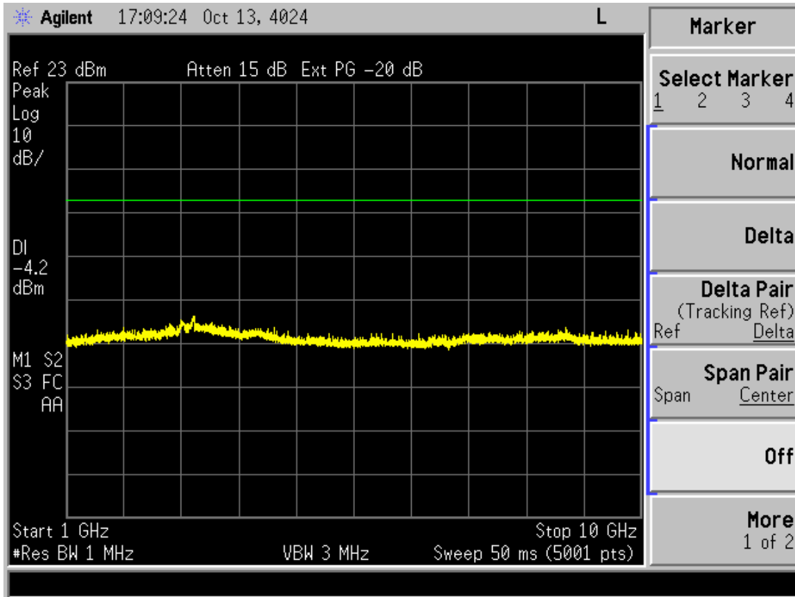
Figure 3. Conducted Spurious Emissions - Low Channel, 1 GHz – 10 GHz
