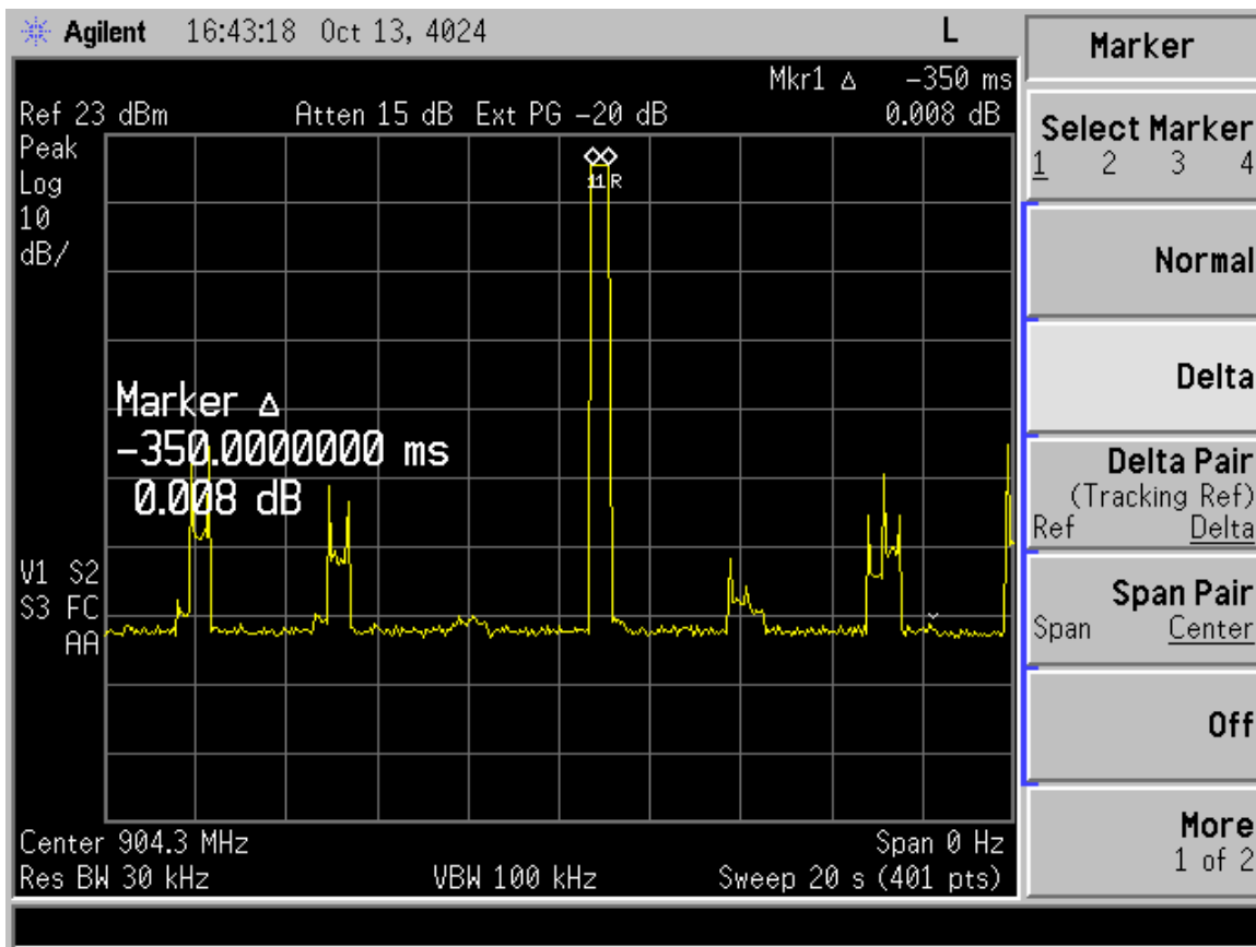
Figure 18. Average Time of Occupancy
