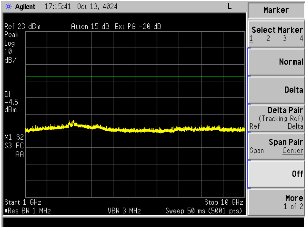
Figure 7. Conducted Spurious Emissions - High Channel, 1 GHz – 10 GHz
