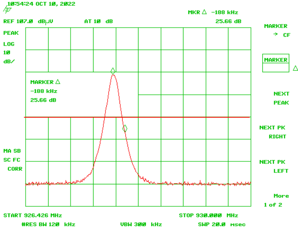
Figure 9. Band Edge Compliance, High Channel Delta – Peak
