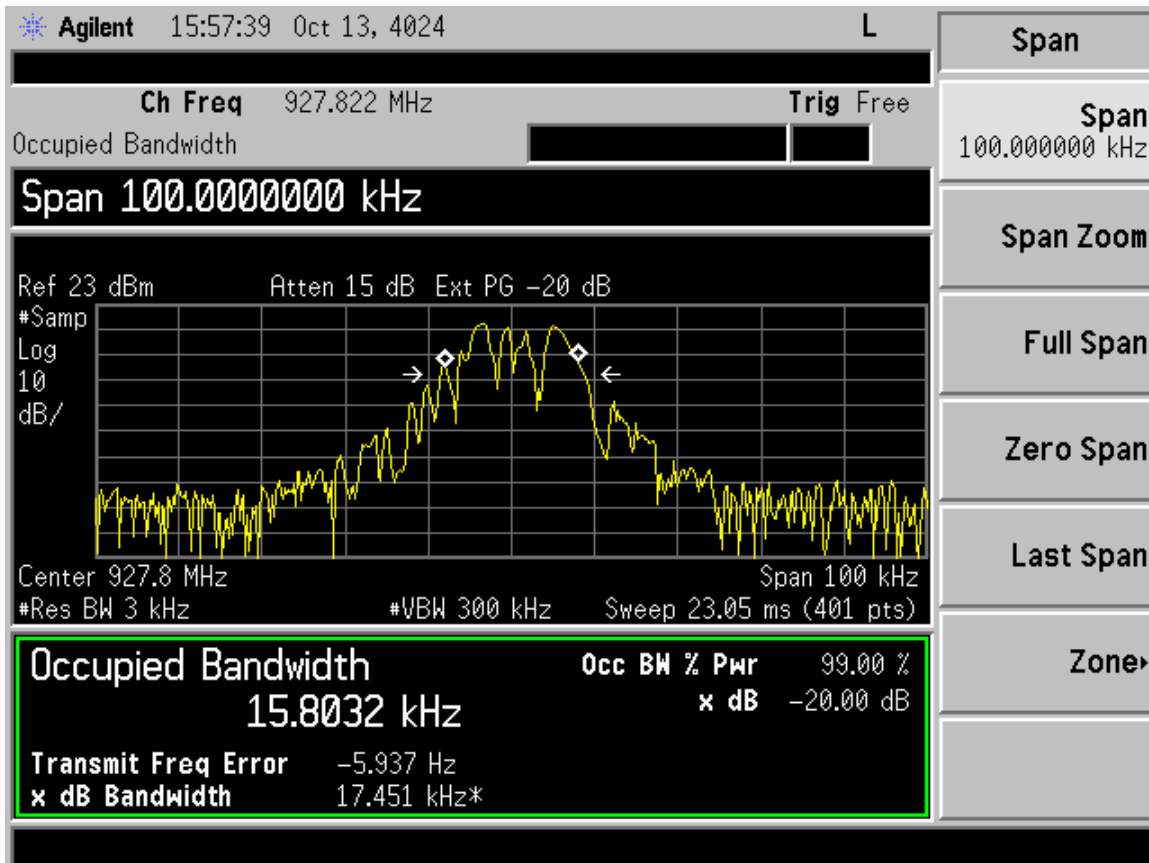
Figure 12. Bandwidth – High Channel
