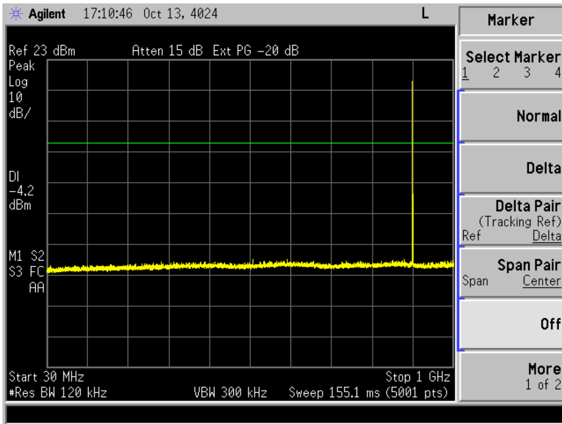
Figure 2. Conducted Spurious Emissions-Low Channel, 30MHz – 1 GHz
