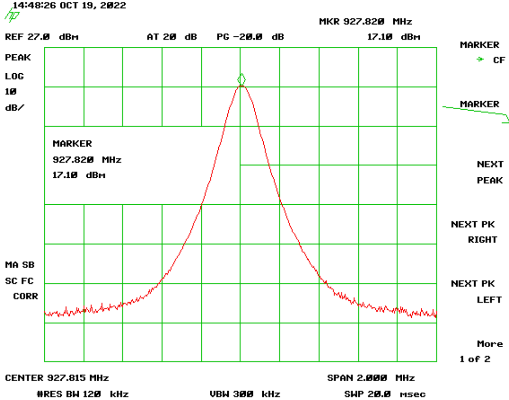
Figure 16. Peak Antenna Conducted Output Power, High Channel
