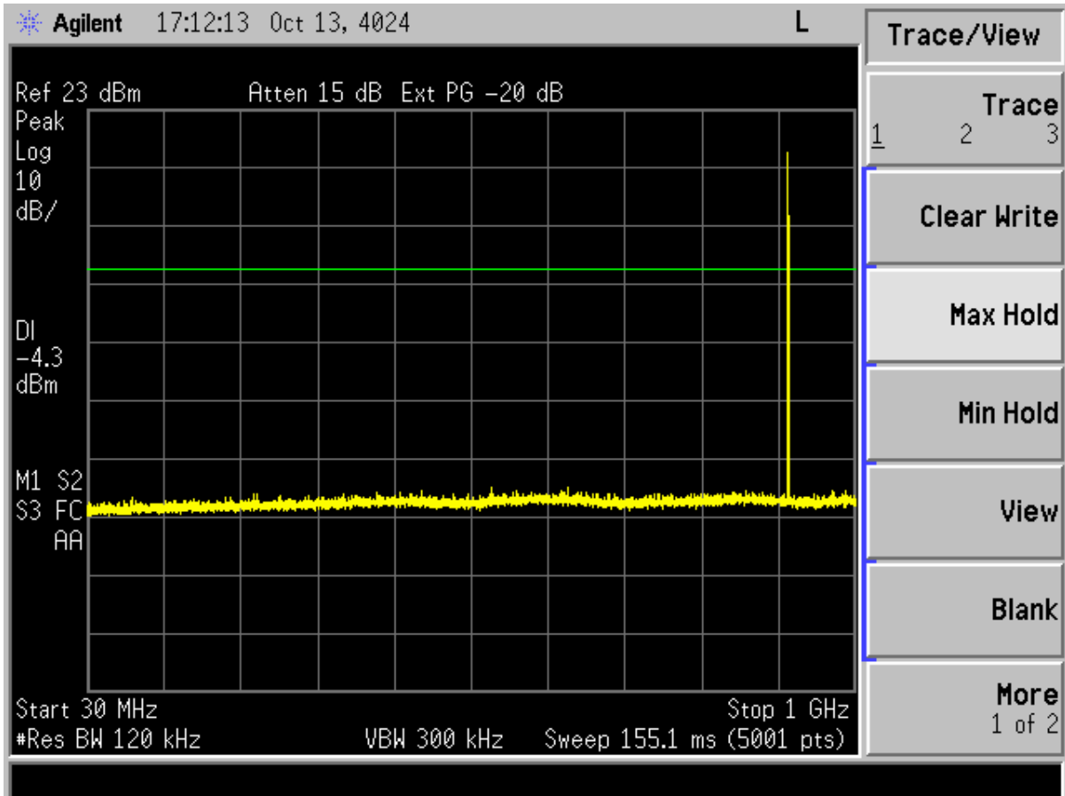
Figure 4. Conducted Spurious Emissions - Mid Channel, 30MHz – 1 GHz
