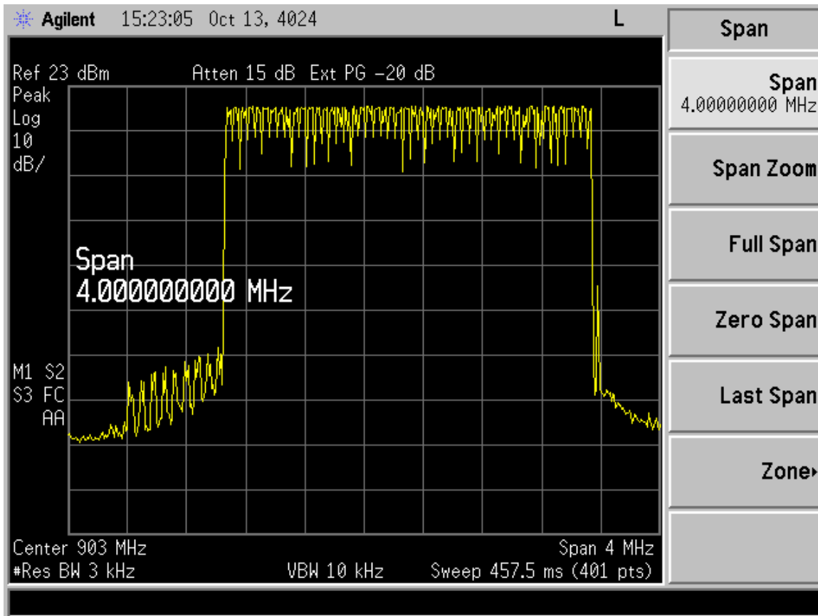
Figure 13. Hopping Channels 0 through 99
