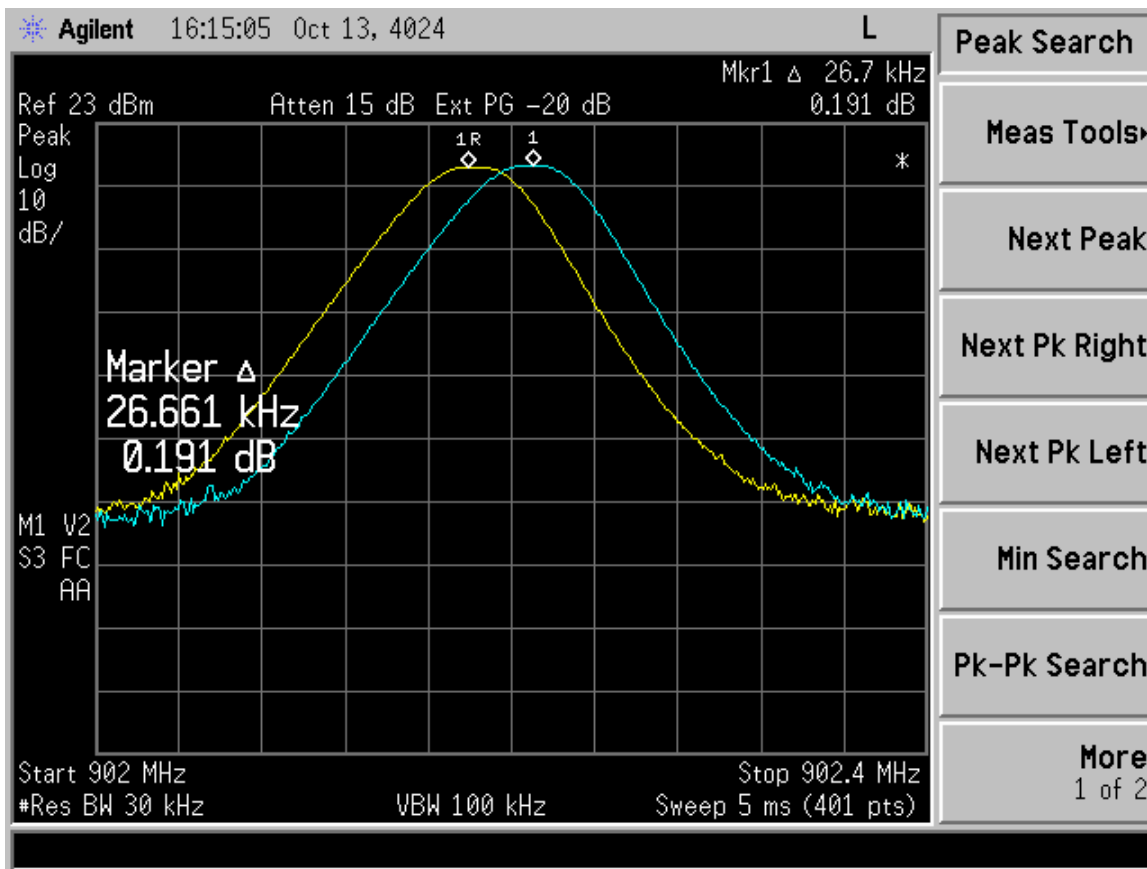
Figure 17. Channel Separation
