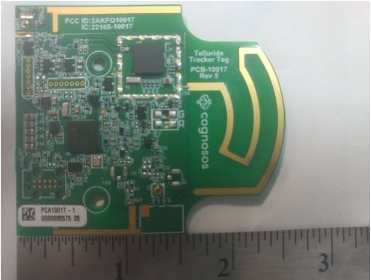
Figure 1. PCB – Front
