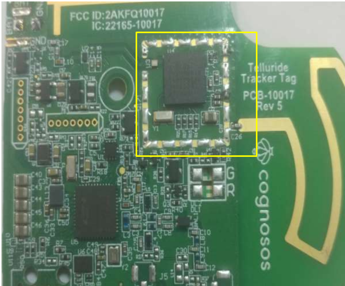
Figure 3. Radio Circuit
