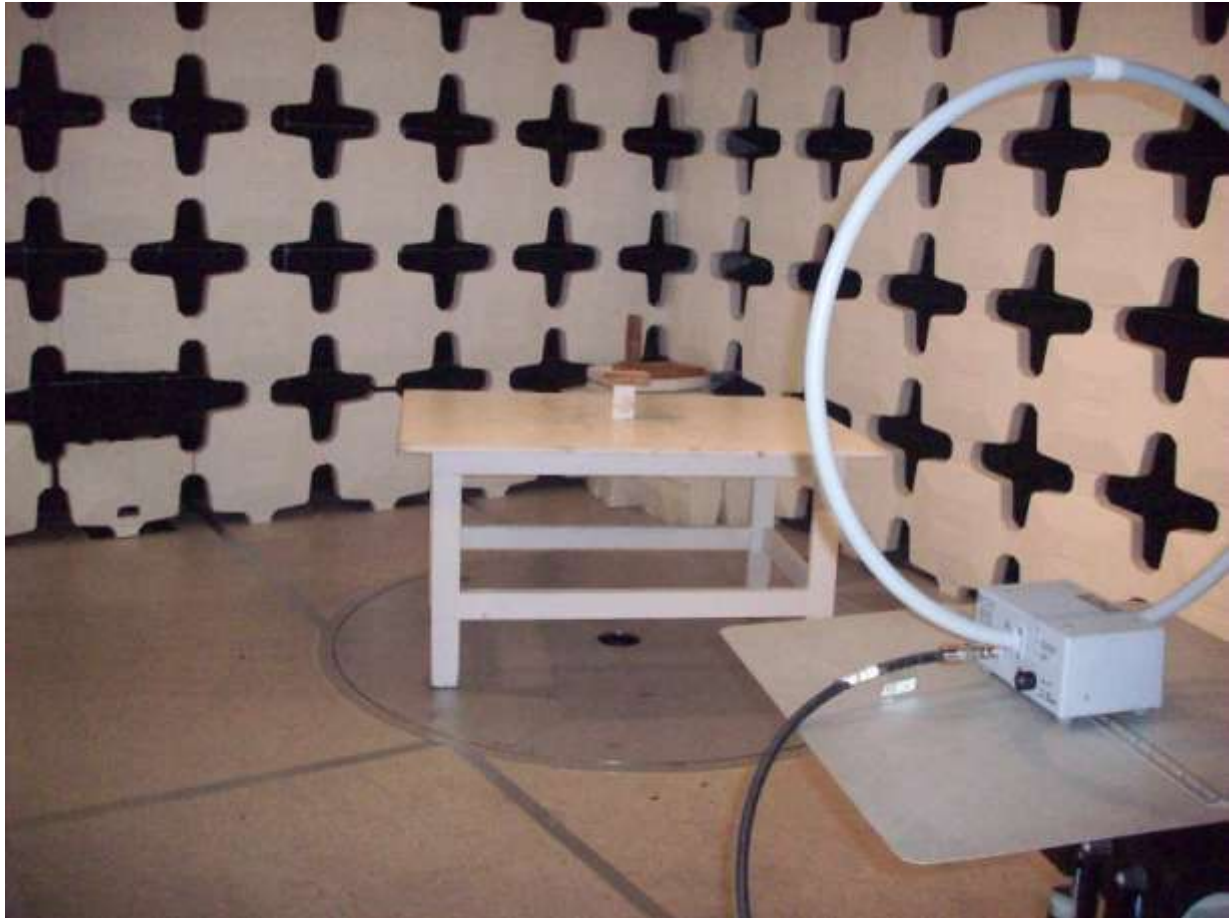
Figure 2. Radiated Emissions Test Setup (9 kHz - 30 MHz)
