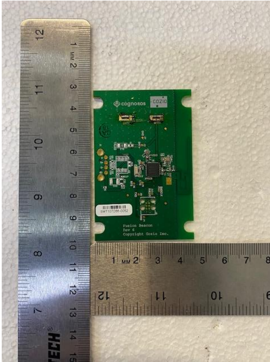
Figure 1. PCB – Front
