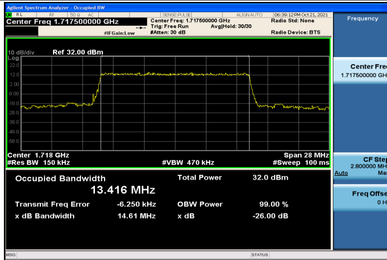
Band4-15MHz-QPSK-20025-75RB#0-13.416
