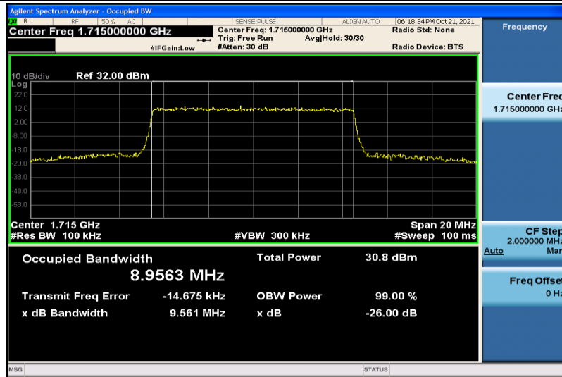
Band4-10MHz-16QAM-20000-50RB#0-8.9563
