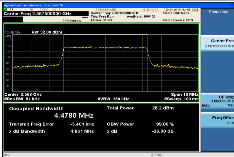
Band7-5MHz-QPSK-21425-25RB#0-4.4780
