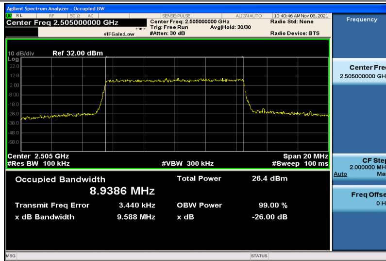
Band7-10MHz-16QAM-20800-50RB#0-8.9386
