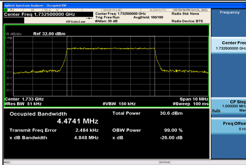
Band4-5MHz-16QAM-20175-25RB#0-4.4741
