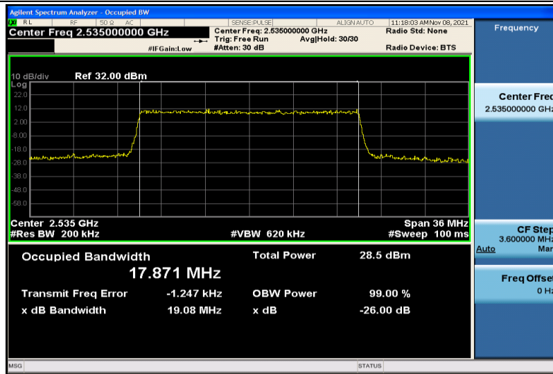
Band7-20MHz-QPSK-21100-100RB#0-17.871
