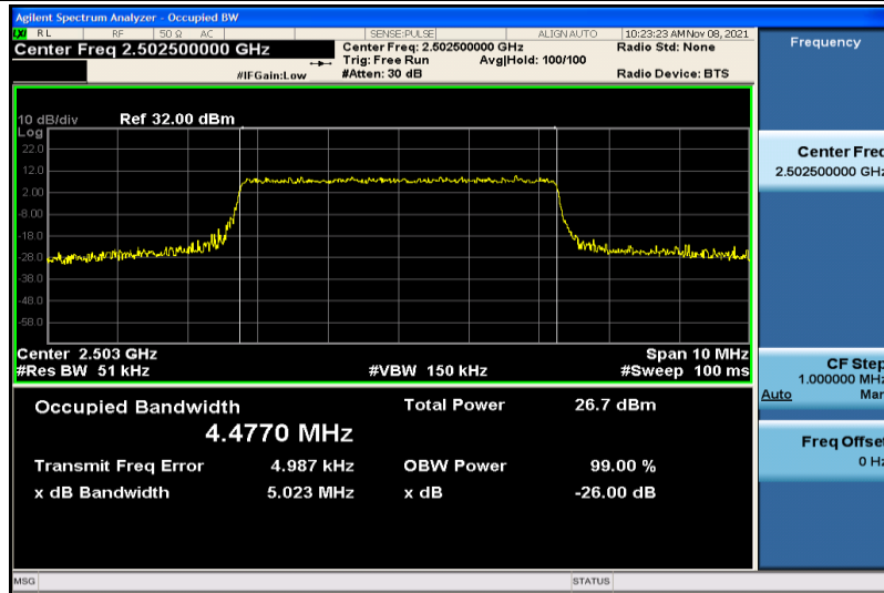
Band7-5MHz-16QAM-20775-25RB#0-4.4770
