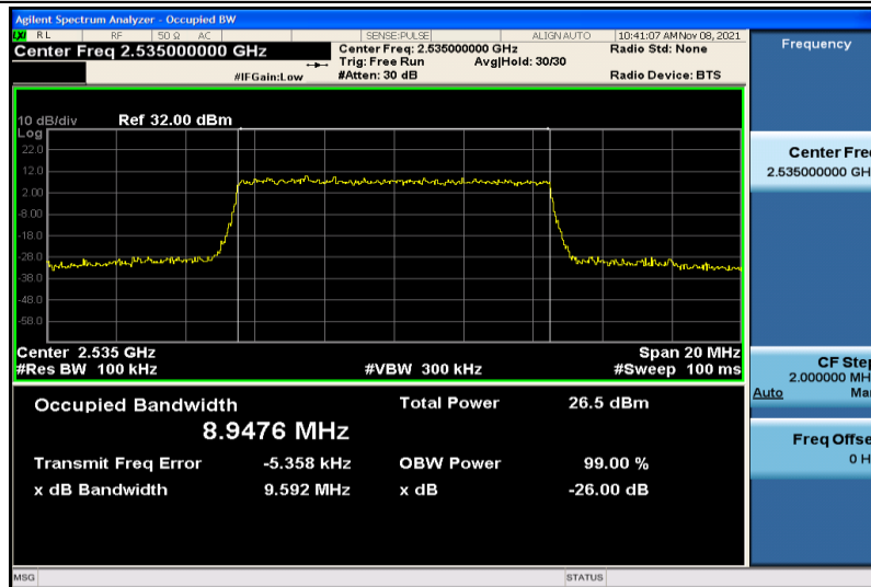
Band7-10MHz-16QAM-21100-50RB#0-8.9476
