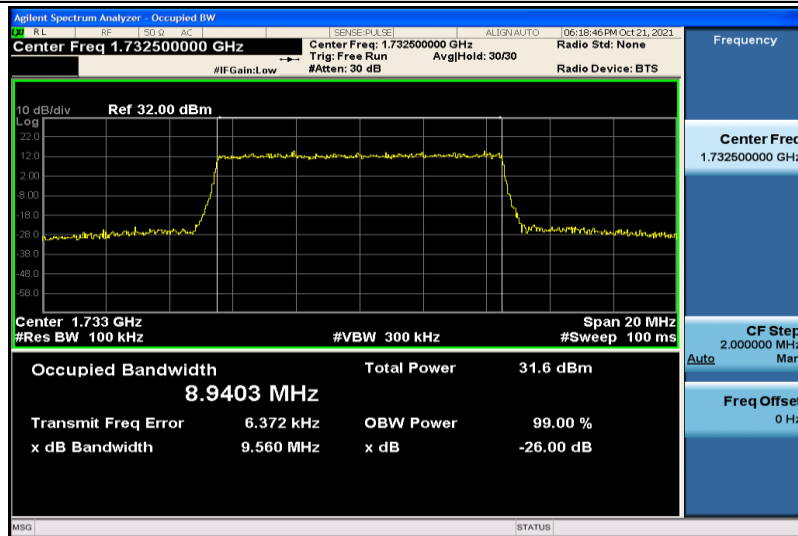
Band4-10MHz-QPSK-20175-50RB#0-8.9403
