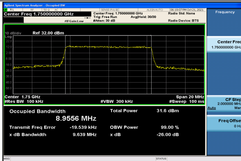
Band4-10MHz-QPSK-20350-50RB#0-8.9556
