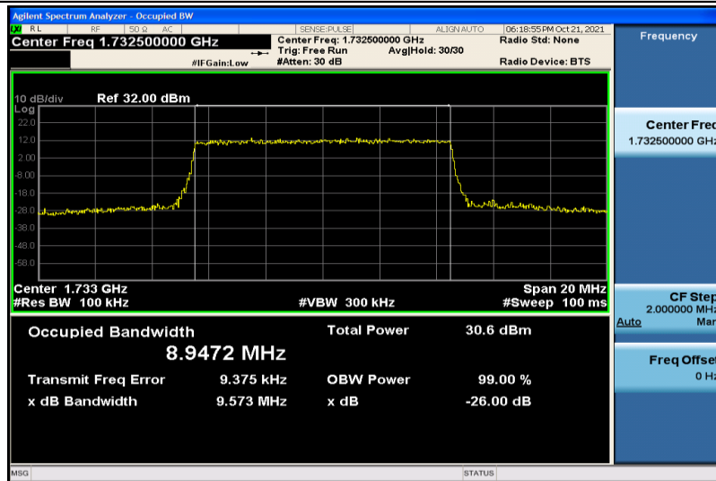
Band4-10MHz-16QAM-20175-50RB#0-8.9472
