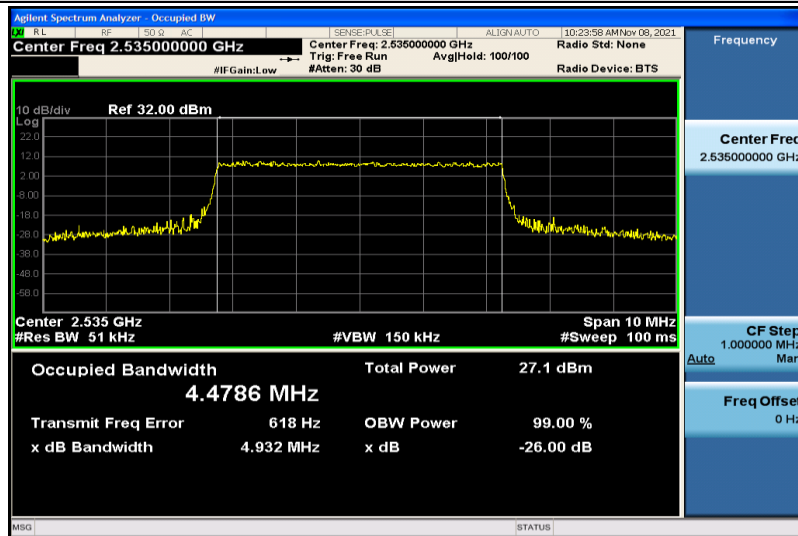
Band7-5MHz-16QAM-21100-25RB#0-4.4786
