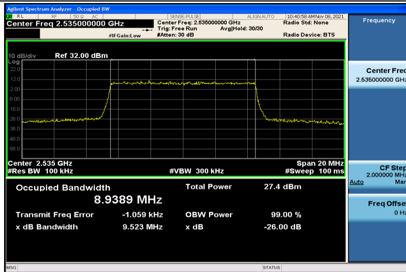
Band7-10MHz-QPSK-21100-50RB#0-8.9389
