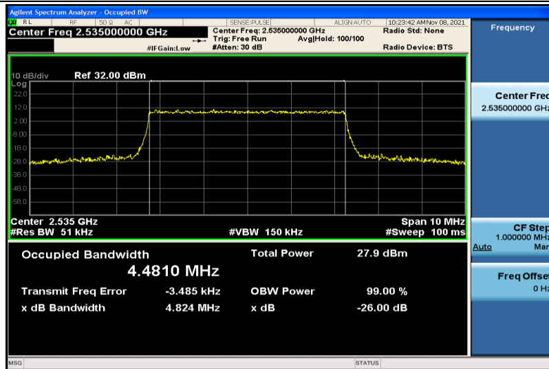
Band7-5MHz-QPSK-21100-25RB#0-4.4810
