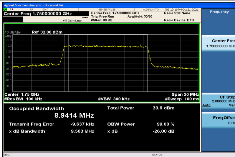
Band4-10MHz-16QAM-20350-50RB#0-8.9414
