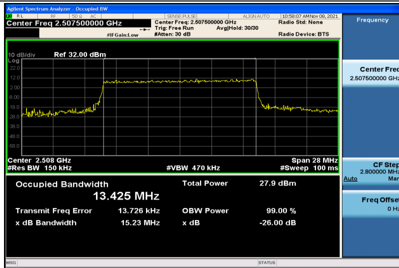
Band7-15MHz-QPSK-20825-75RB#0-13.425
