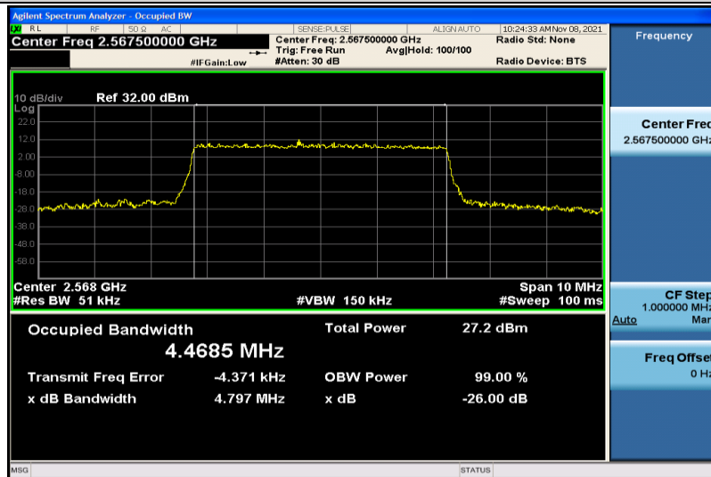
Band7-5MHz-16QAM-21425-25RB#0-4.4685
