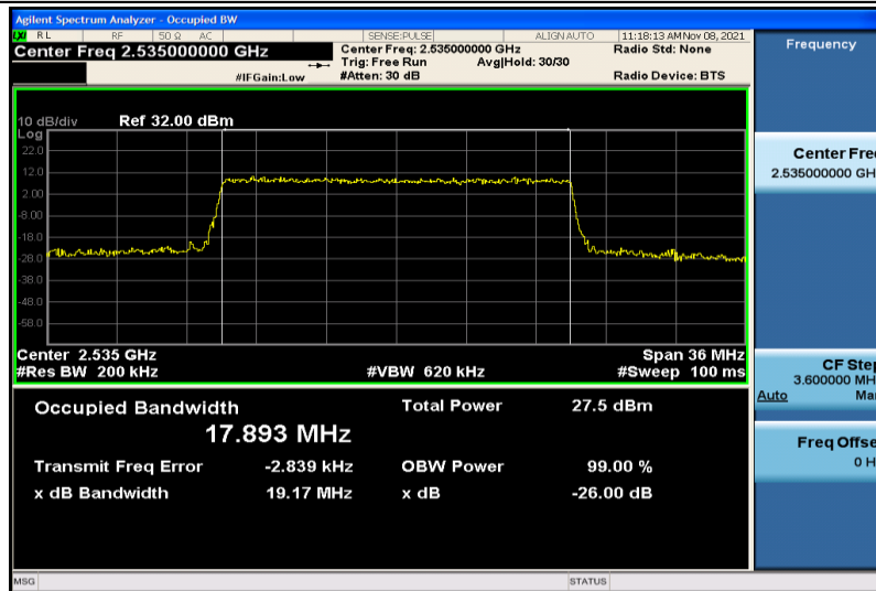
Band7-20MHz-16QAM-21100-100RB#0-17.893
