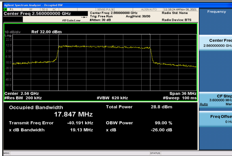
Band7-20MHz-QPSK-21350-100RB#0-17.847
