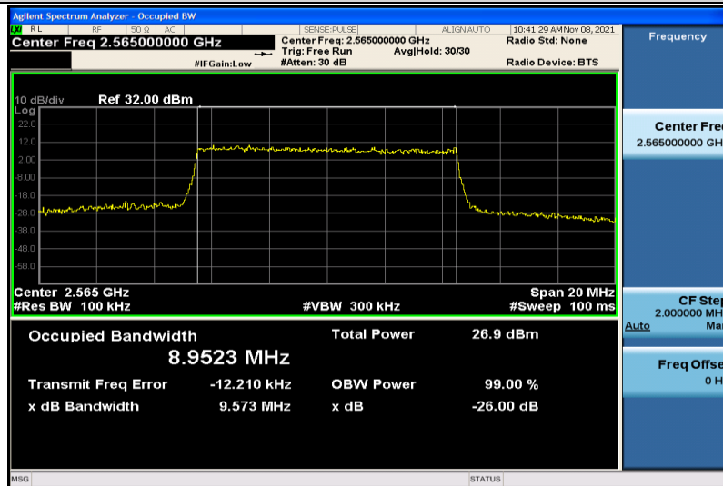
Band7-10MHz-16QAM-21400-50RB#0-8.9523
