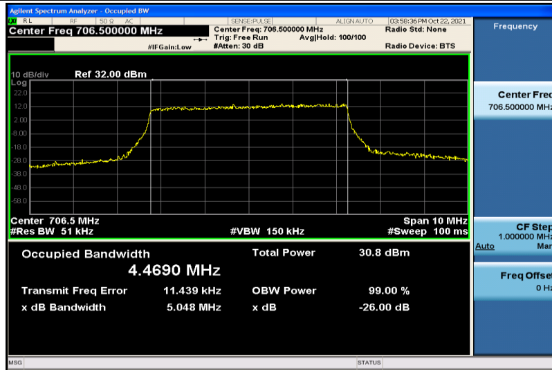
Band17-5MHz-QPSK-23755-25RB#0-4.4690
