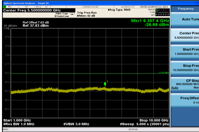
GPRS850-190-1000~10000
