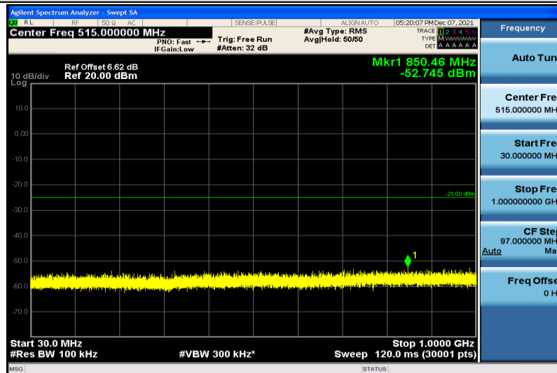
Band7-5MHz-16QAM-20775-1RB#0-30~1000MHz
