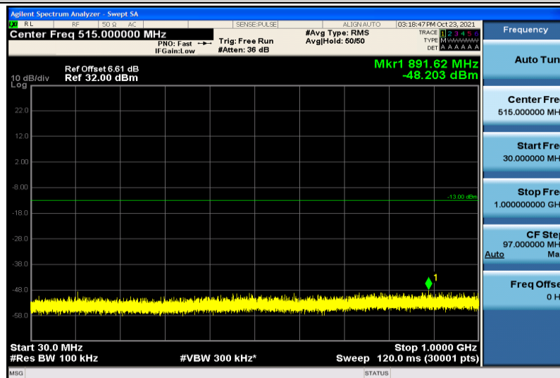
Band4-10MHz-16QAM-20175-1RB#0-30~1000MHz
