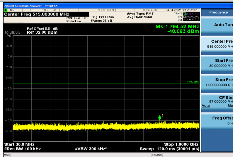
Band4-20MHz-16QAM-20175-1RB#0-30~1000MHz
