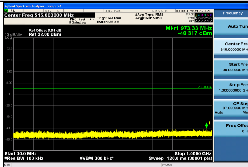
Band4-10MHz-QPSK-20175-1RB#0-30~1000MHz
