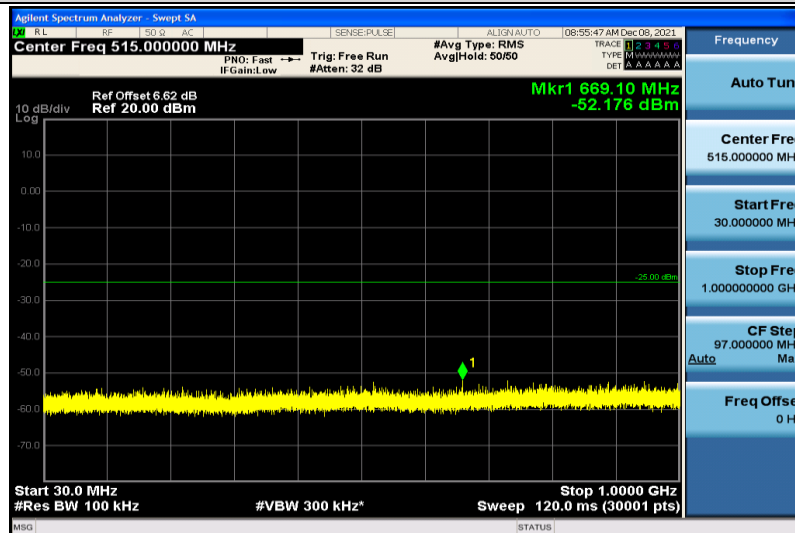
Band7-15MHz-QPSK-20825-1RB#0-30~1000MHz
