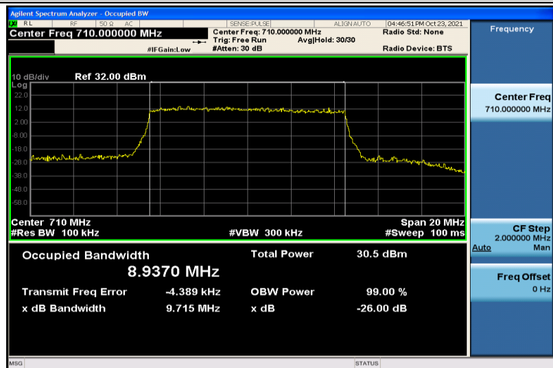
Band17-10MHz-16QAM-23790-50RB#0-8.9370
