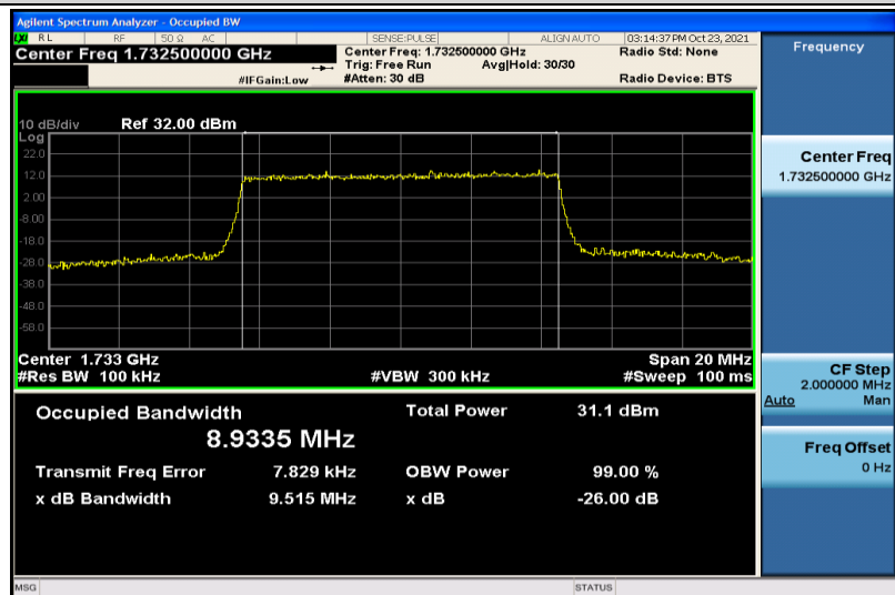
Band4-10MHz-QPSK-20175-50RB#0-8.9335
