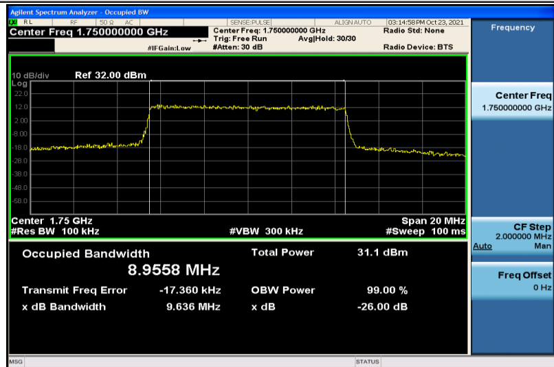
Band4-10MHz-QPSK-20350-50RB#0-8.9558
