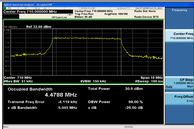
Band17-5MHz-16QAM-23790-25RB#0-4.4788
