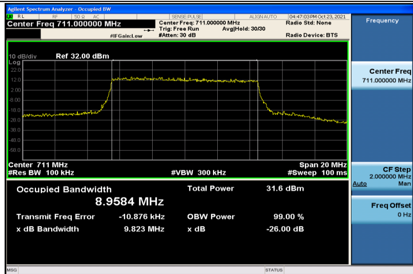
Band17-10MHz-QPSK-23800-50RB#0-8.9584
