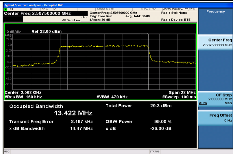
Band7-15MHz-QPSK-20825-75RB#0-13.422
