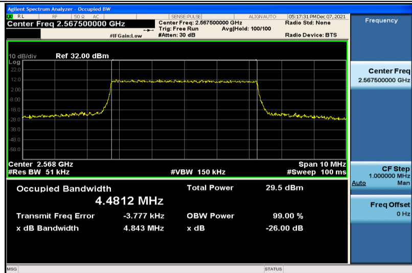
Band7-5MHz-QPSK-21425-25RB#0-4.4812
