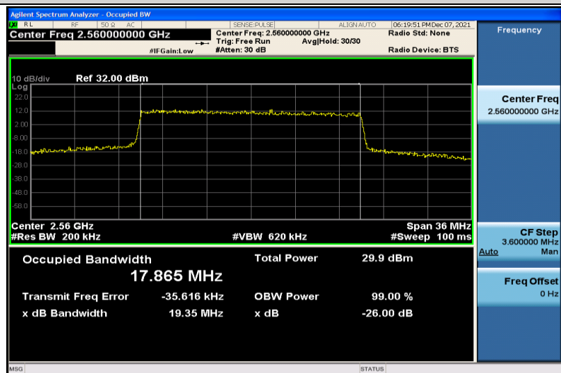
Band7-20MHz-QPSK-21350-100RB#0-17.865
