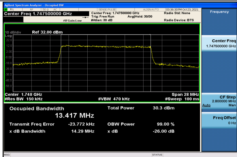
Band4-15MHz-16QAM-20325-75RB#0-13.417
