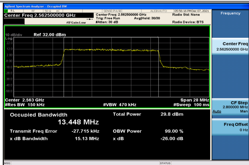
Band7-15MHz-QPSK-21375-75RB#0-13.448
