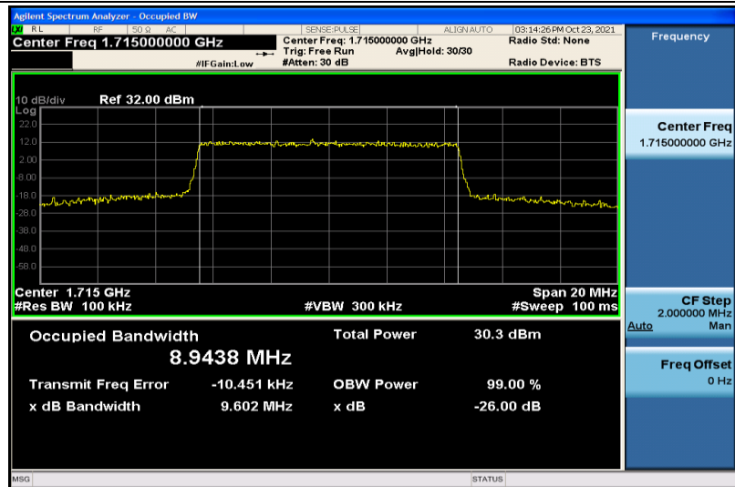
Band4-10MHz-16QAM-20000-50RB#0-8.9438
