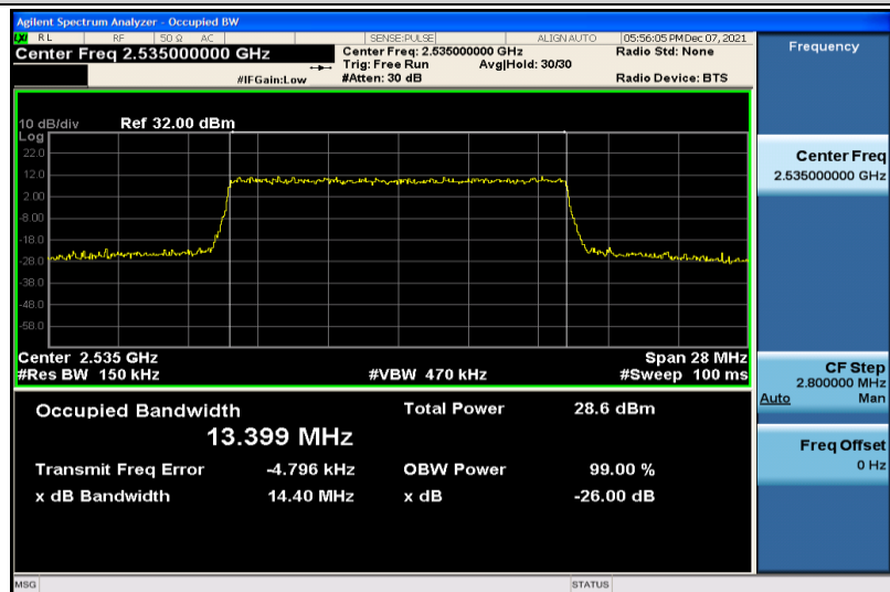
Band7-15MHz-16QAM-21100-75RB#0-13.399
