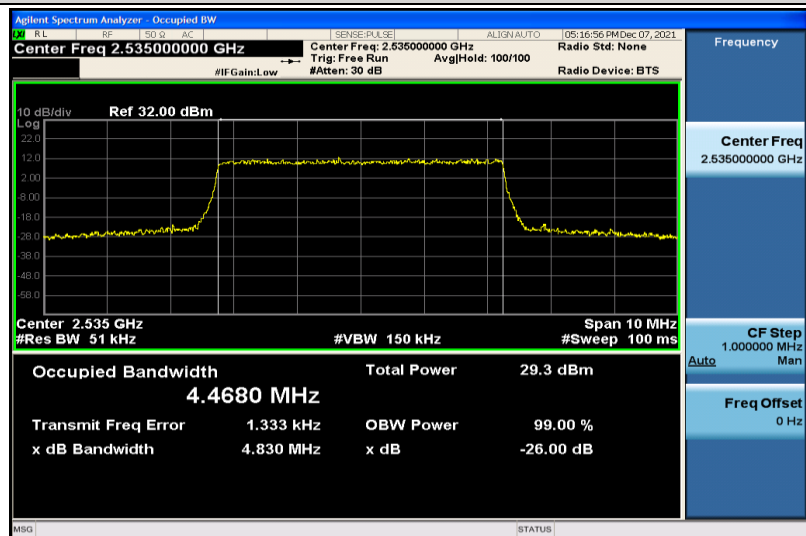
Band7-5MHz-QPSK-21100-25RB#0-4.4680
