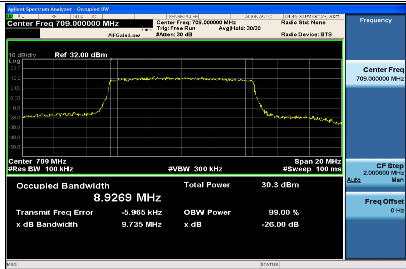
Band17-10MHz-16QAM-23780-50RB#0-8.9269
