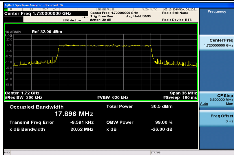
Band4-20MHz-QPSK-20050-100RB#0-17.896
