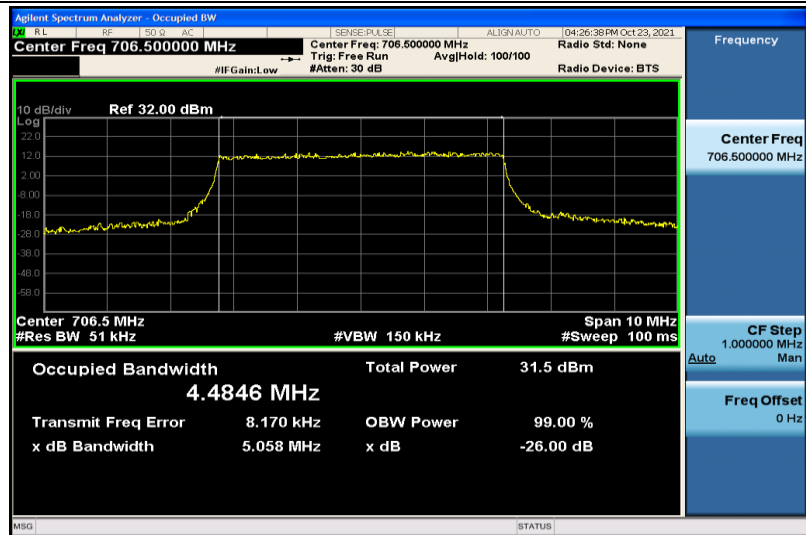
Band17-5MHz-QPSK-23755-25RB#0-4.4846
