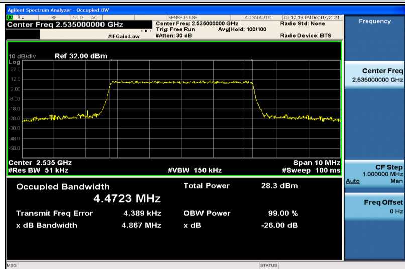
Band7-5MHz-16QAM-21100-25RB#0-4.4723
