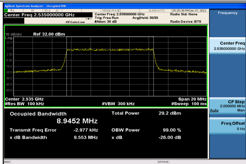
Band7-10MHz-QPSK-21100-50RB#0-8.9452
