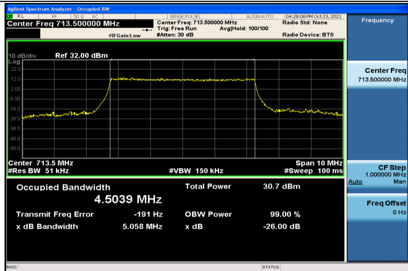
Band17-5MHz-16QAM-23825-25RB#0-4.5039
