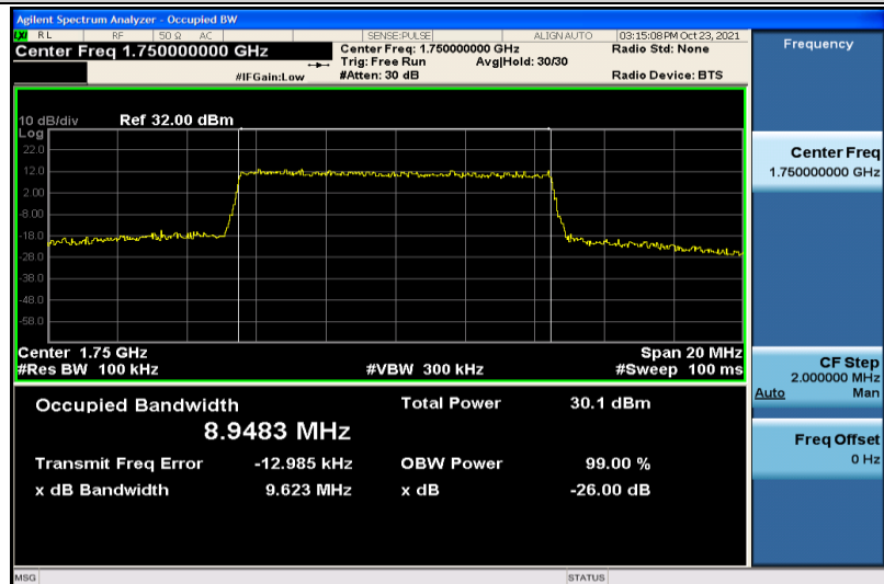
Band4-10MHz-16QAM-20350-50RB#0-8.9483
