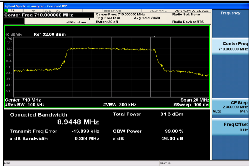
Band17-10MHz-QPSK-23790-50RB#0-8.9448
