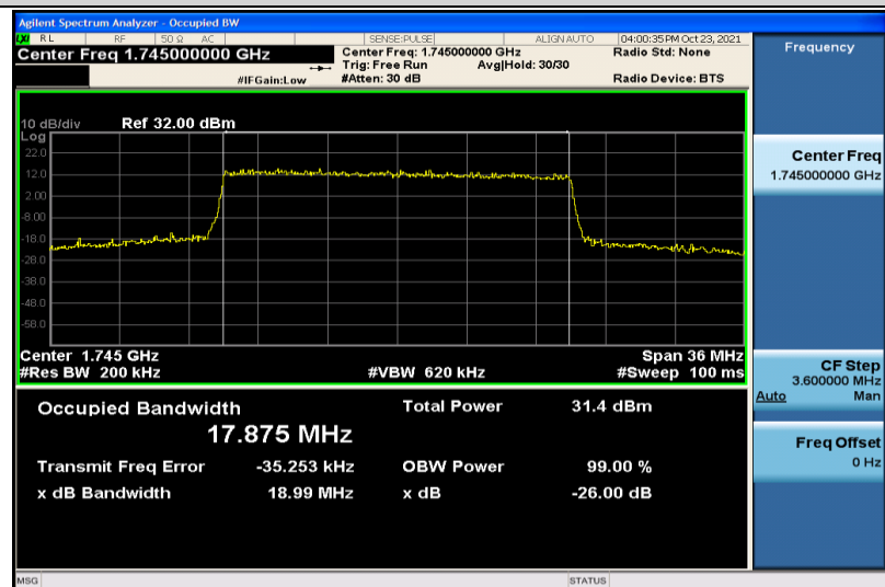
Band4-20MHz-QPSK-20300-100RB#0-17.875
