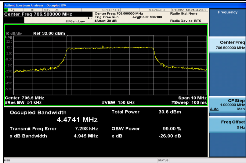
Band17-5MHz-16QAM-23755-25RB#0-4.4741
