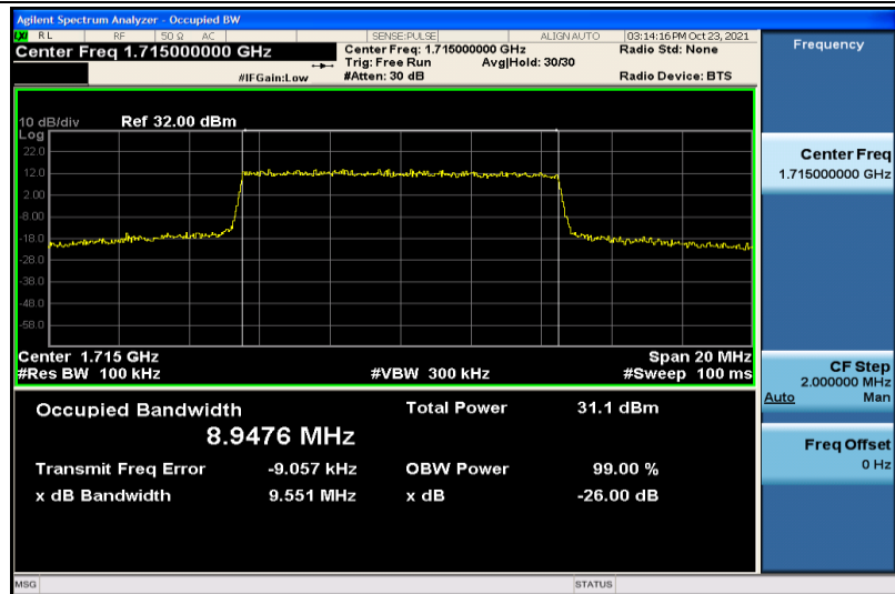
Band4-10MHz-QPSK-20000-50RB#0-8.9476
