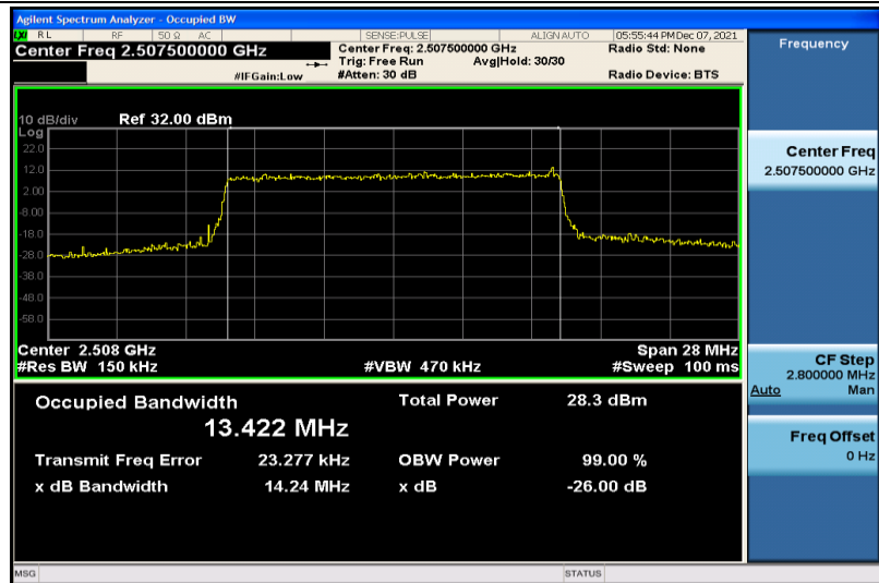
Band7-15MHz-16QAM-20825-75RB#0-13.422
