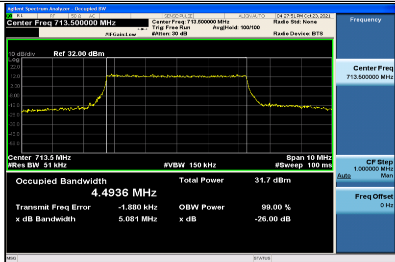
Band17-5MHz-QPSK-23825-25RB#0-4.4936
