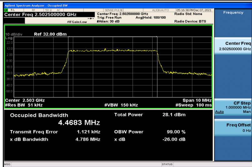
Band7-5MHz-16QAM-20775-25RB#0-4.4683
