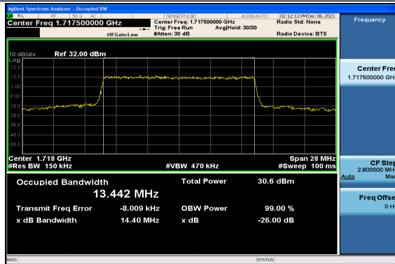
Band4-15MHz-QPSK-20025-75RB#0-13.442
