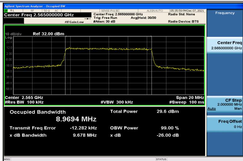
Band7-10MHz-QPSK-21400-50RB#0-8.9694
