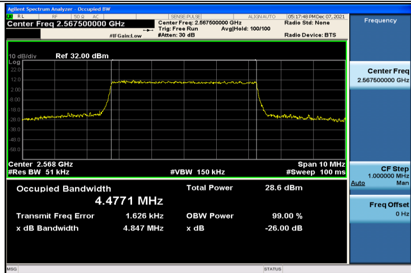
Band7-5MHz-16QAM-21425-25RB#0-4.4771
