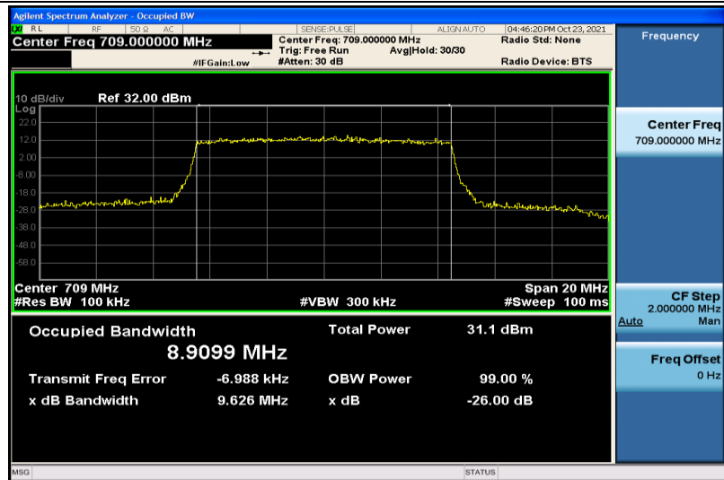
Band17-10MHz-QPSK-23780-50RB#0-8.9099
