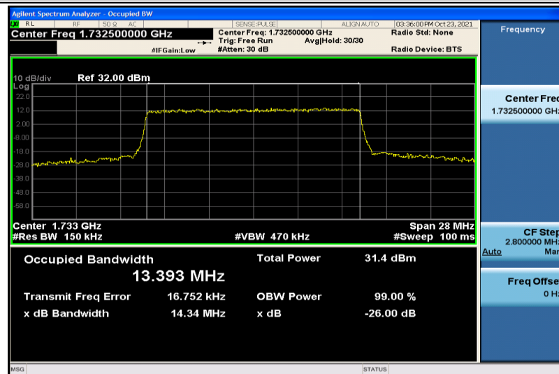
Band4-15MHz-QPSK-20175-75RB#0-13.393
