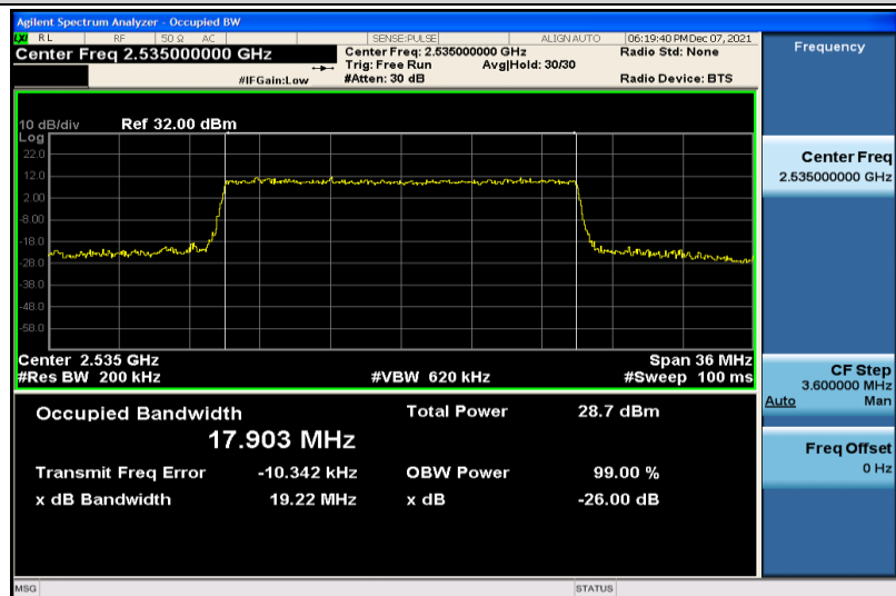
Band7-20MHz-16QAM-21100-100RB#0-17.903
