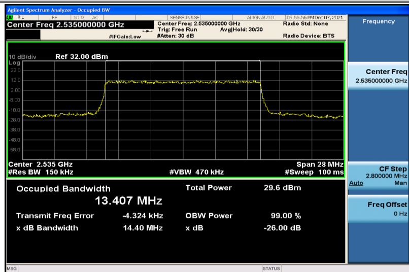
Band7-15MHz-QPSK-21100-75RB#0-13.407
