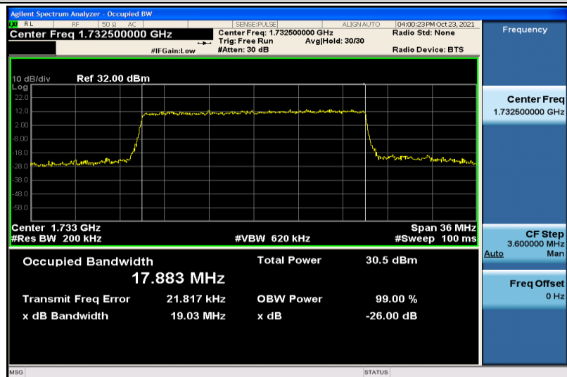
Band4-20MHz-16QAM-20175-100RB#0-17.883
