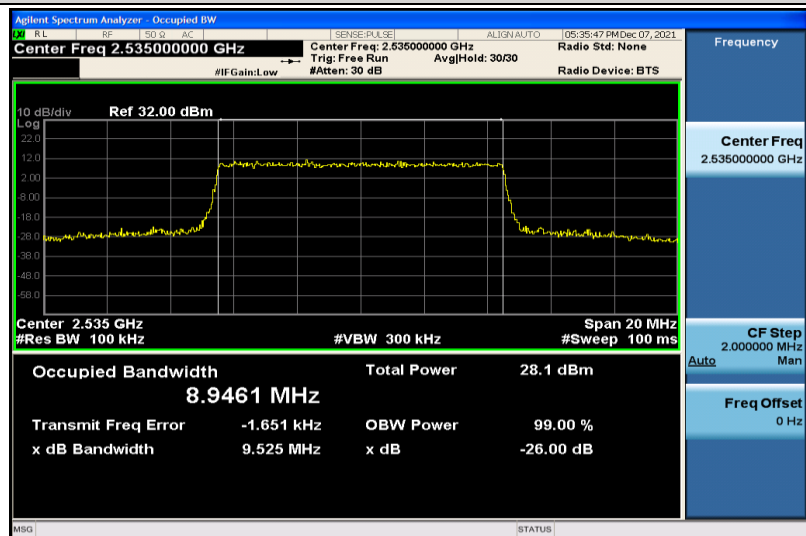
Band7-10MHz-16QAM-21100-50RB#0-8.9461
