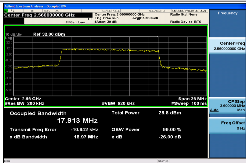
Band7-20MHz-16QAM-21350-100RB#0-17.913
