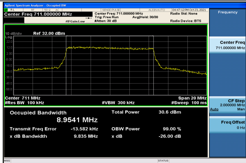
Band17-10MHz-16QAM-23800-50RB#0-8.9541
