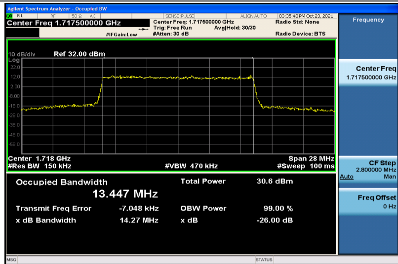
Band4-15MHz-16QAM-20025-75RB#0-13.447
