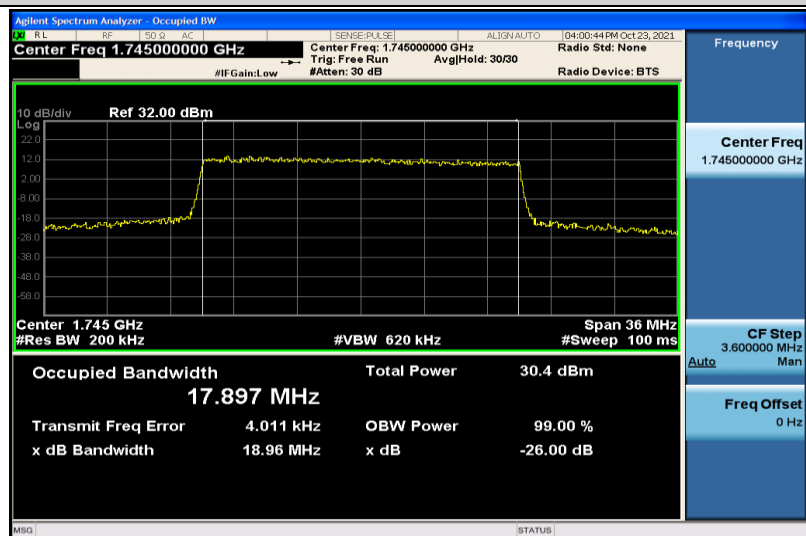
Band4-20MHz-16QAM-20300-100RB#0-17.897
