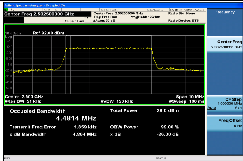
Band7-5MHz-QPSK-20775-25RB#0-4.4814
