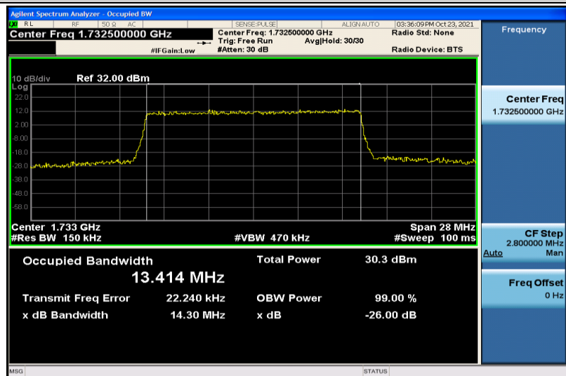
Band4-15MHz-16QAM-20175-75RB#0-13.414
