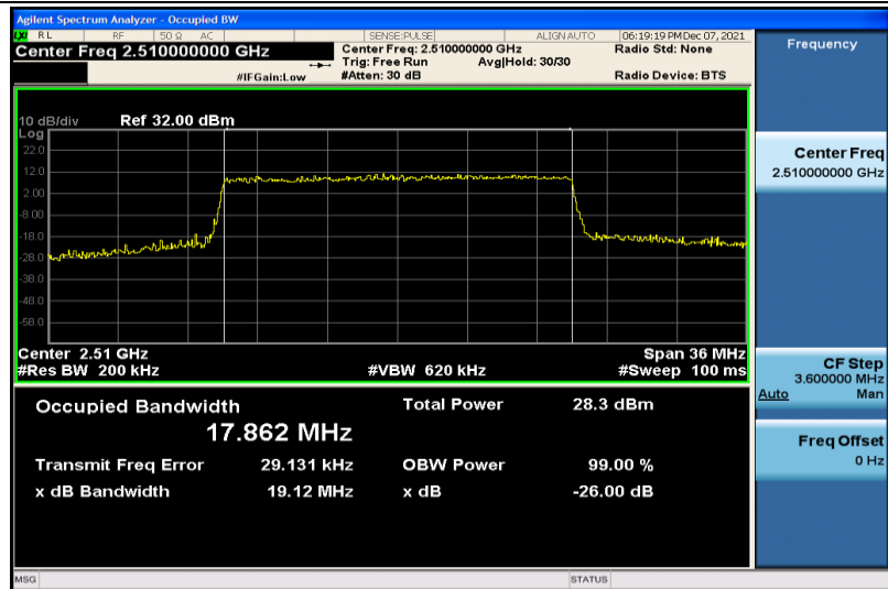
Band7-20MHz-16QAM-20850-100RB#0-17.862
