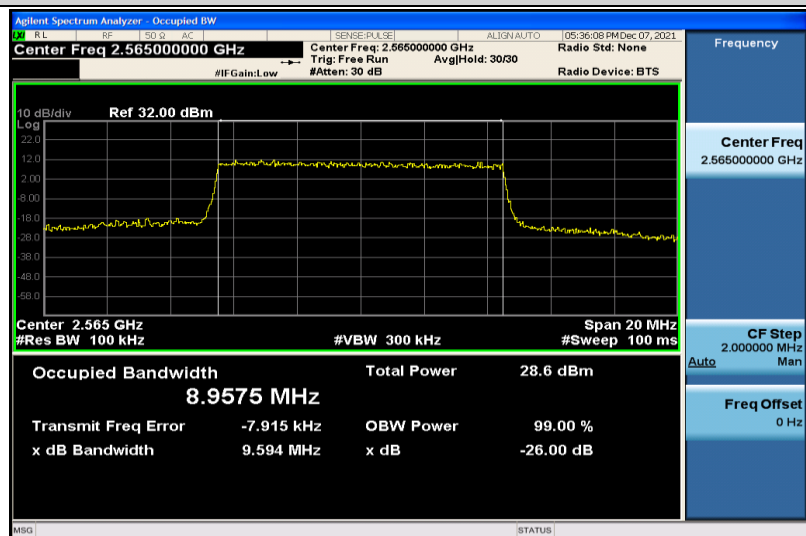
Band7-10MHz-16QAM-21400-50RB#0-8.9575
