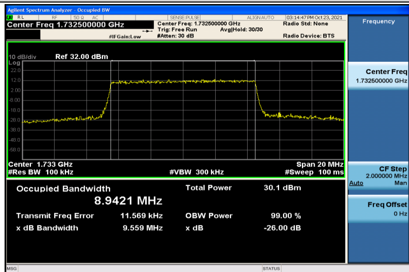
Band4-10MHz-16QAM-20175-50RB#0-8.9421
