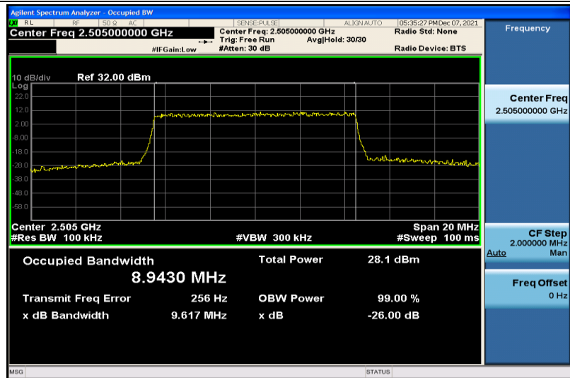
Band7-10MHz-16QAM-20800-50RB#0-8.9430
