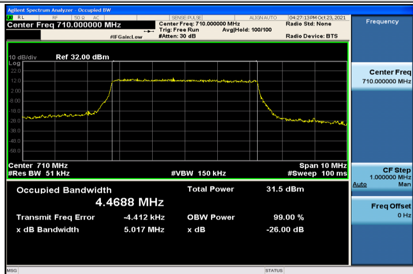
Band17-5MHz-QPSK-23790-25RB#0-4.4688
