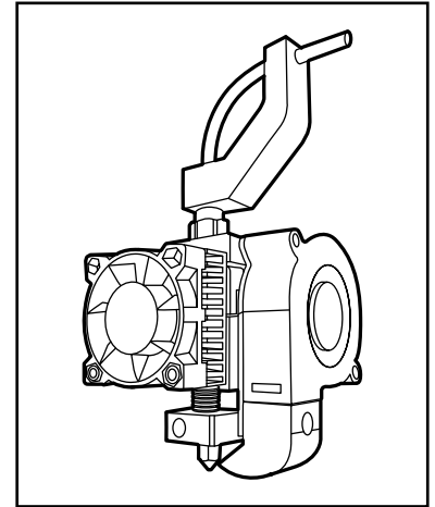
Figure 5.1 Witbox extruder
