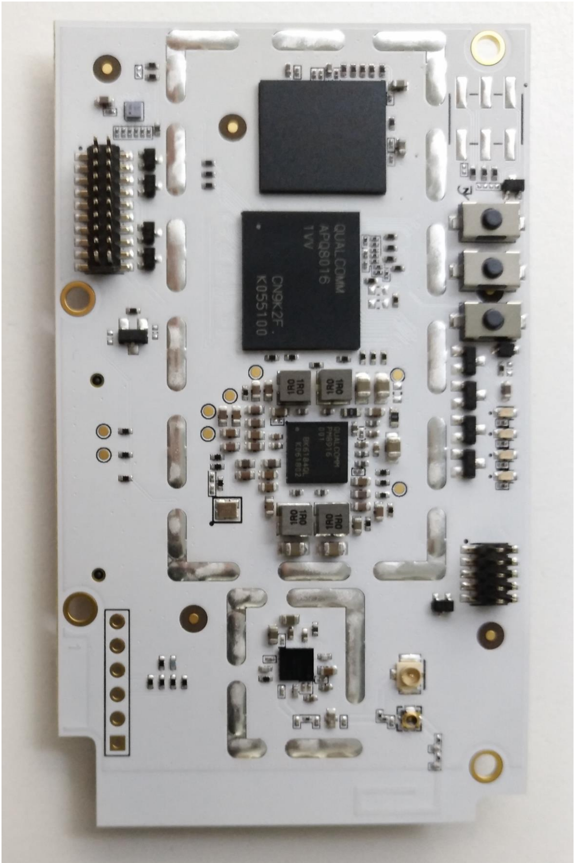
QC410 Board top view
