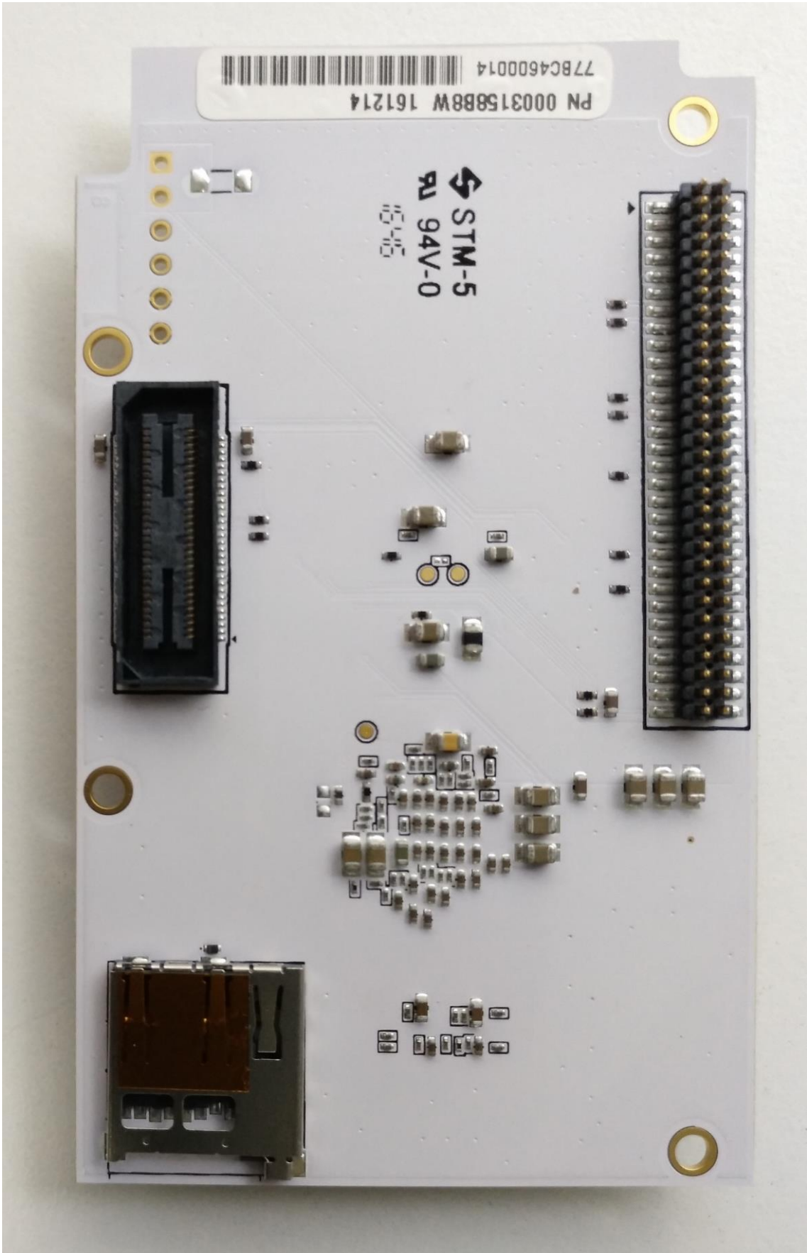
QC410 Board bottom view
