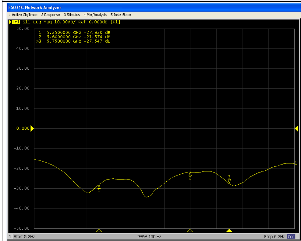
Return Loss for Head TSL
