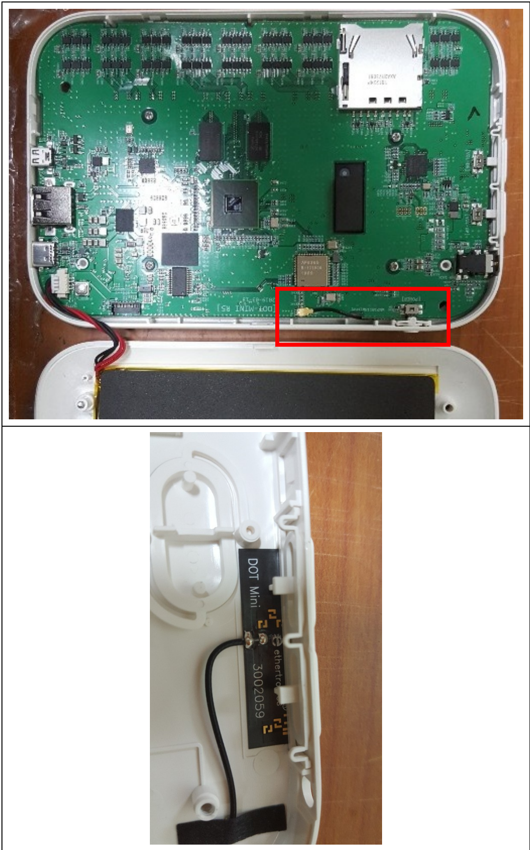
Antenna Photo
