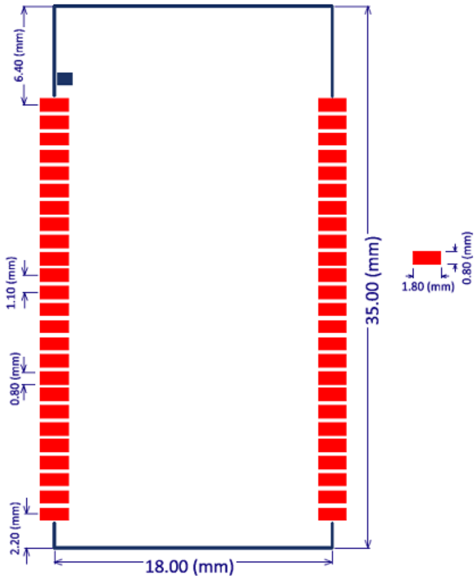
Figure 5. Footprint dimensions
