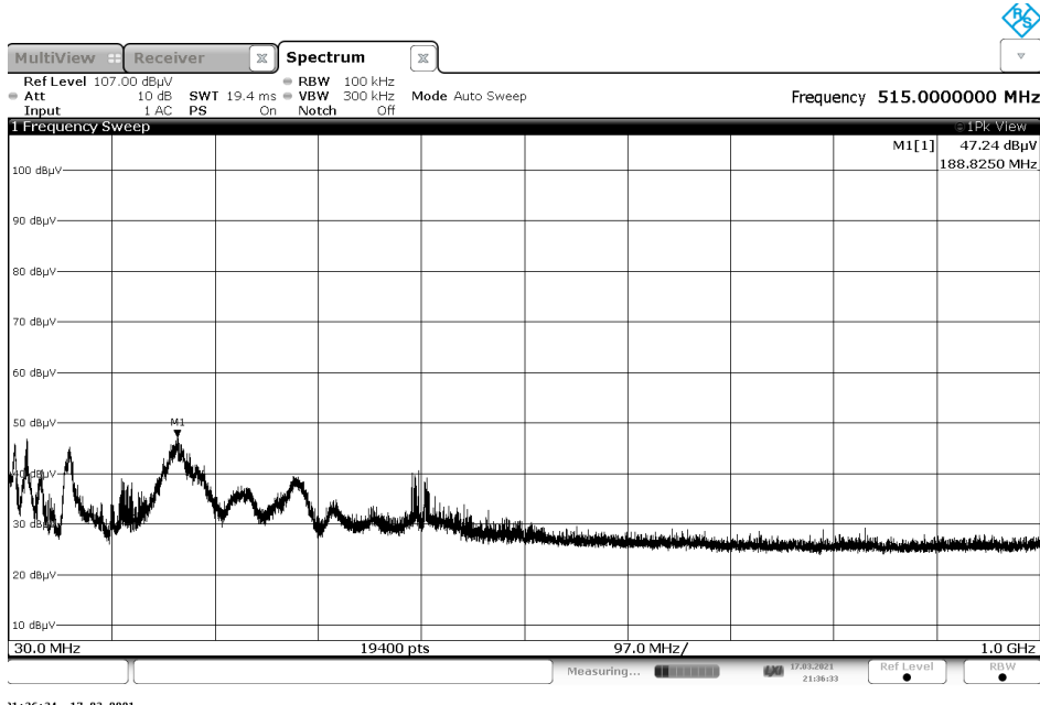
Note: Emissions above the noise floor are not associated with the radio. Figure A-3: 30MHz-1GHz
