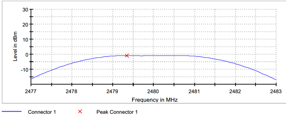
Figure 7.4.2-4: 2480MHz Plot
