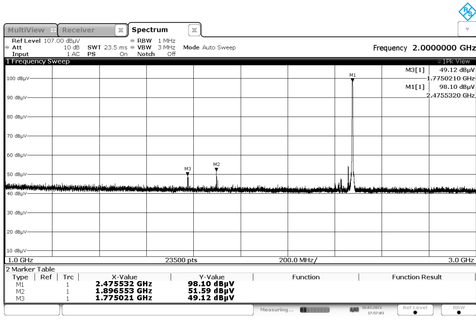
Note: Emissions above the noise floor are not associated with the radio, except fundamental emission. Figure A-4: 1GHz-3GHz
