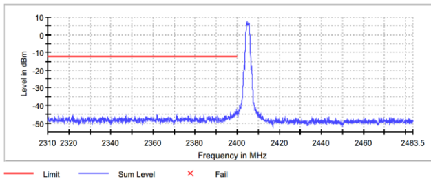
Figure 7.5.1.2-5: Lower Band-edge
