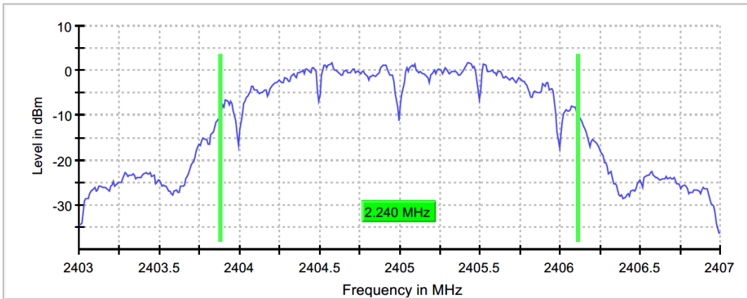
Figure 7.3.2-5: 2405MHz - 99% OBW
