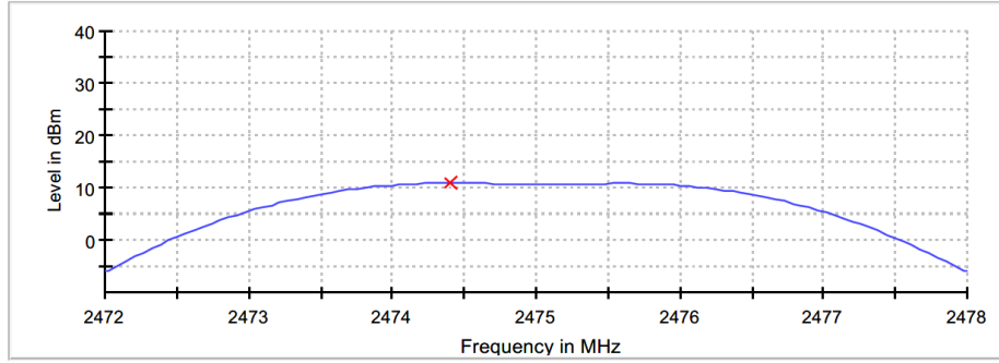
Figure 7.4.2-3: 2475MHz Plot
