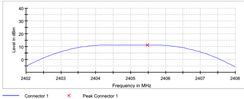
Figure 7.4.2-1: 2405MHz Plot
