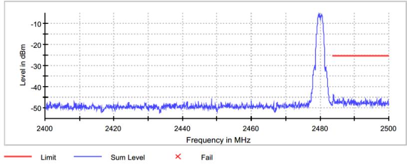
Figure 7.5.1.2-7: Upper Band-edge (2480MHz)
