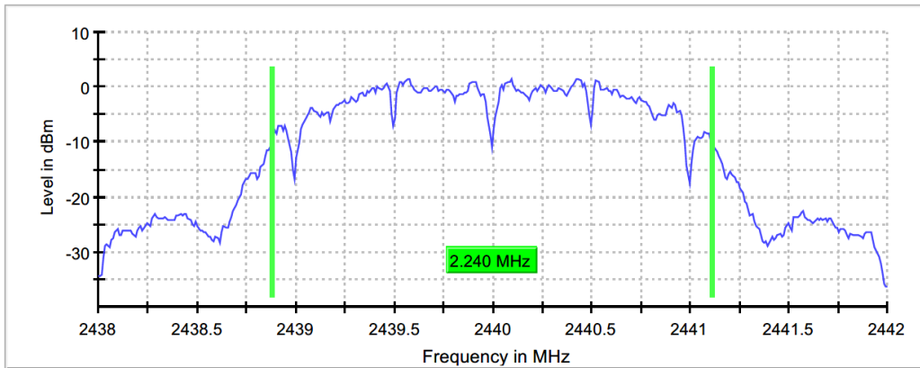
Figure 7.3.2-6: 2440MHz - 99% OBW
