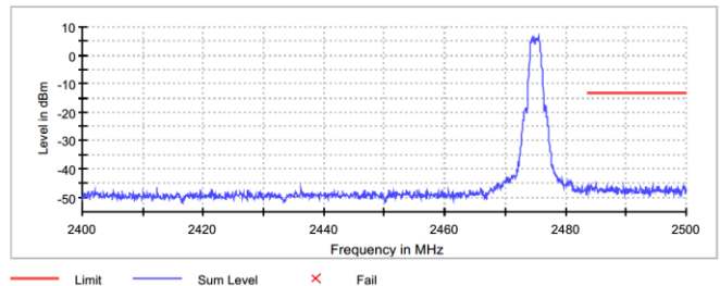
Figure 7.5.1.2-6: Upper Band-edge (2475MHz)
