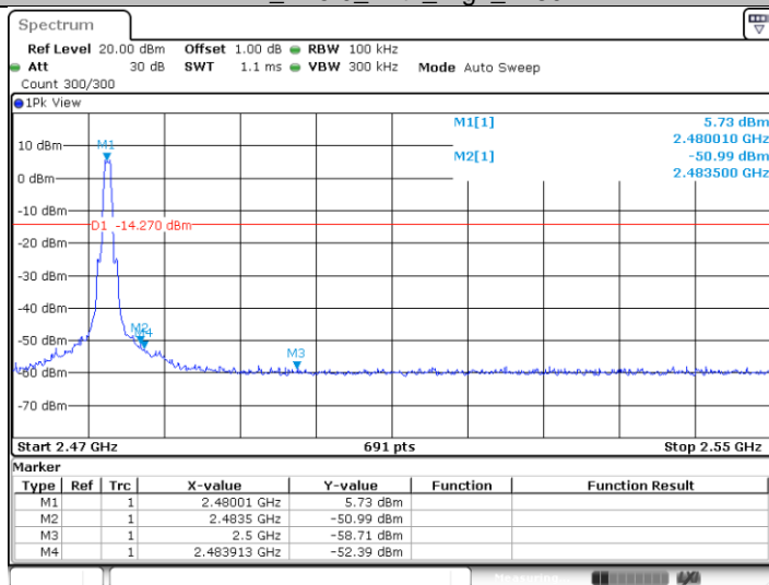
BLE_BT5.0_Ant1_High_2480
