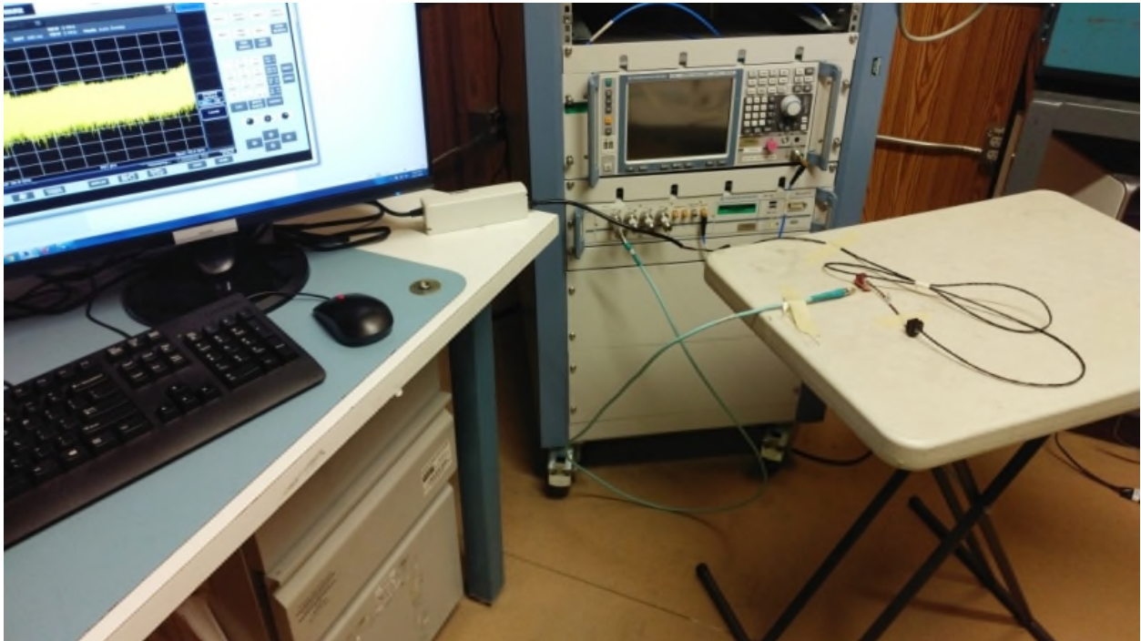
Figure 1: Equipment Under Test – Radiated Emissions – Antenna Port Conducted Measurements
