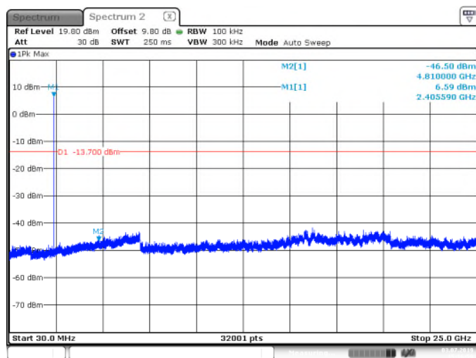
Figure 7.5.1.2-1: LCH – 30MHz–25GHz
