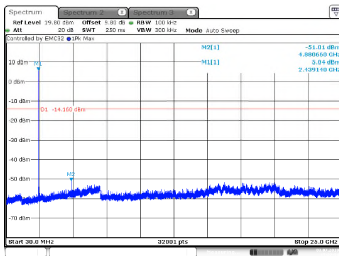
Figure 7.5.1.2-2: MCH – 30MHz–25GHz
