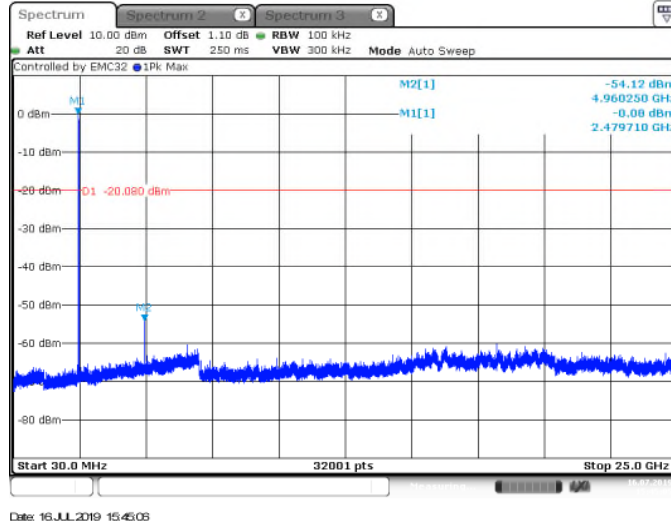
Figure 7.5.1.2-3: HCH – 30MHz–25GHz
