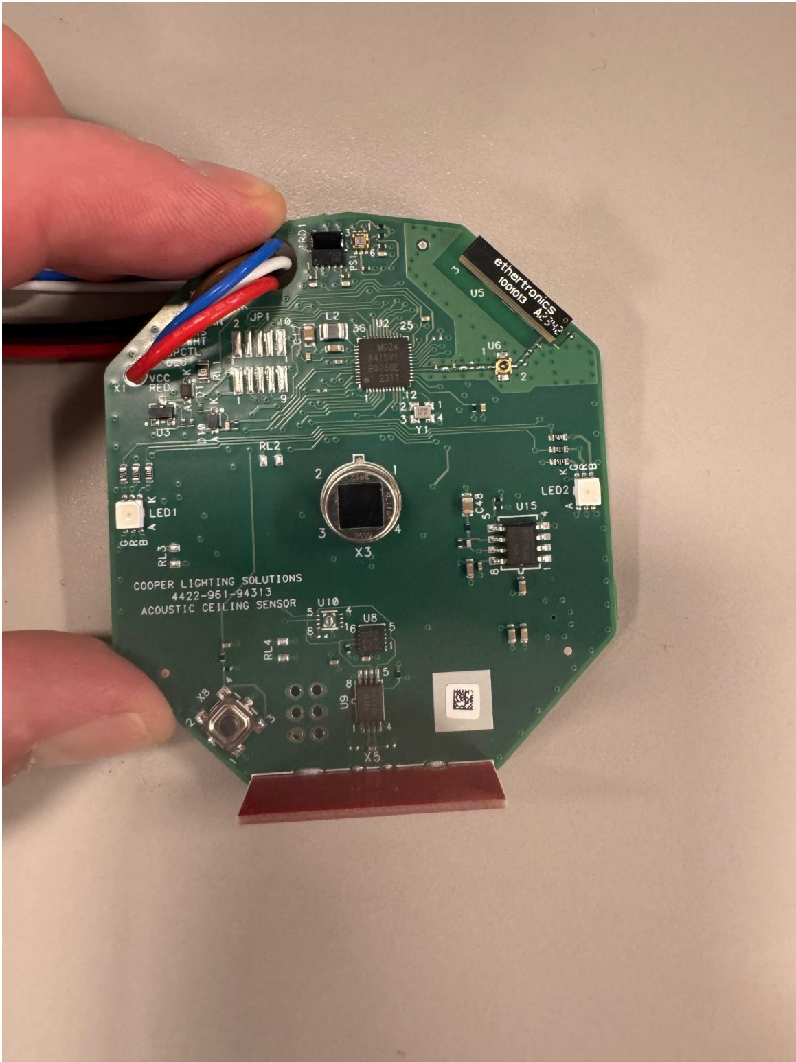
Figure 3: Low Voltage Top
