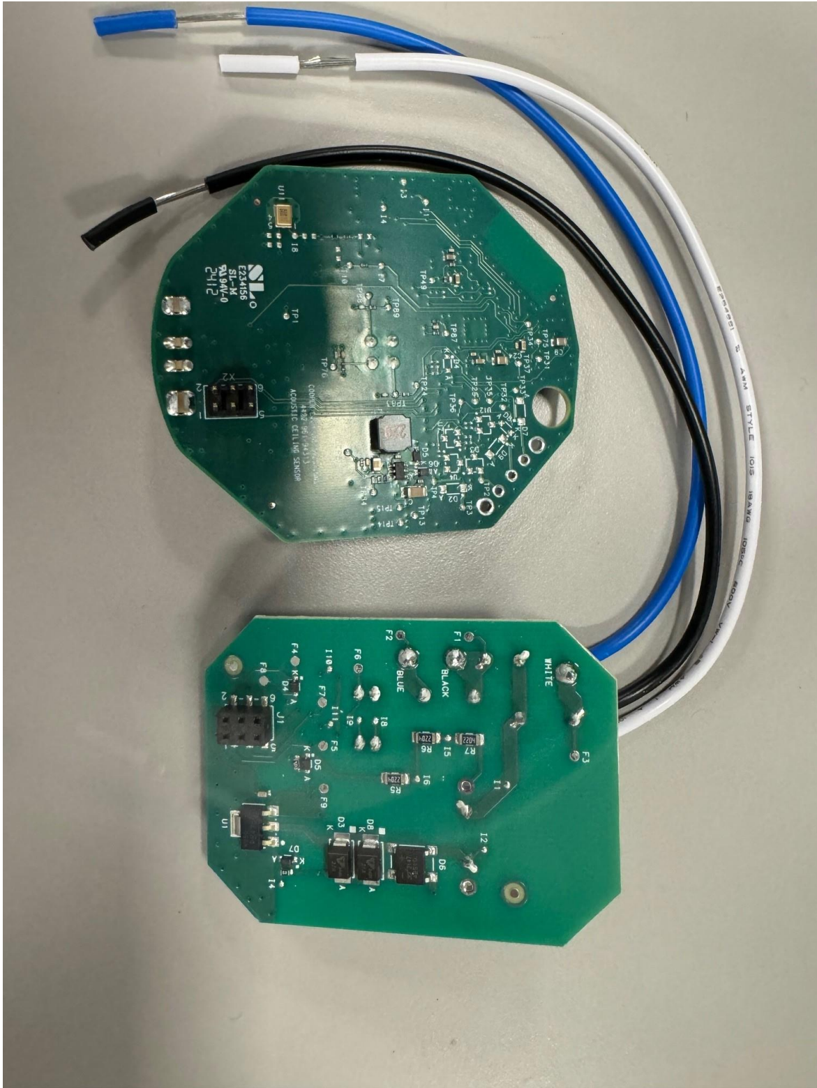
Figure 2: Line Voltage Bottom
