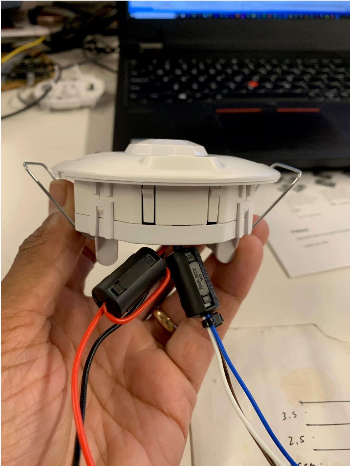
Figure 6: Low Voltage Side View 1
