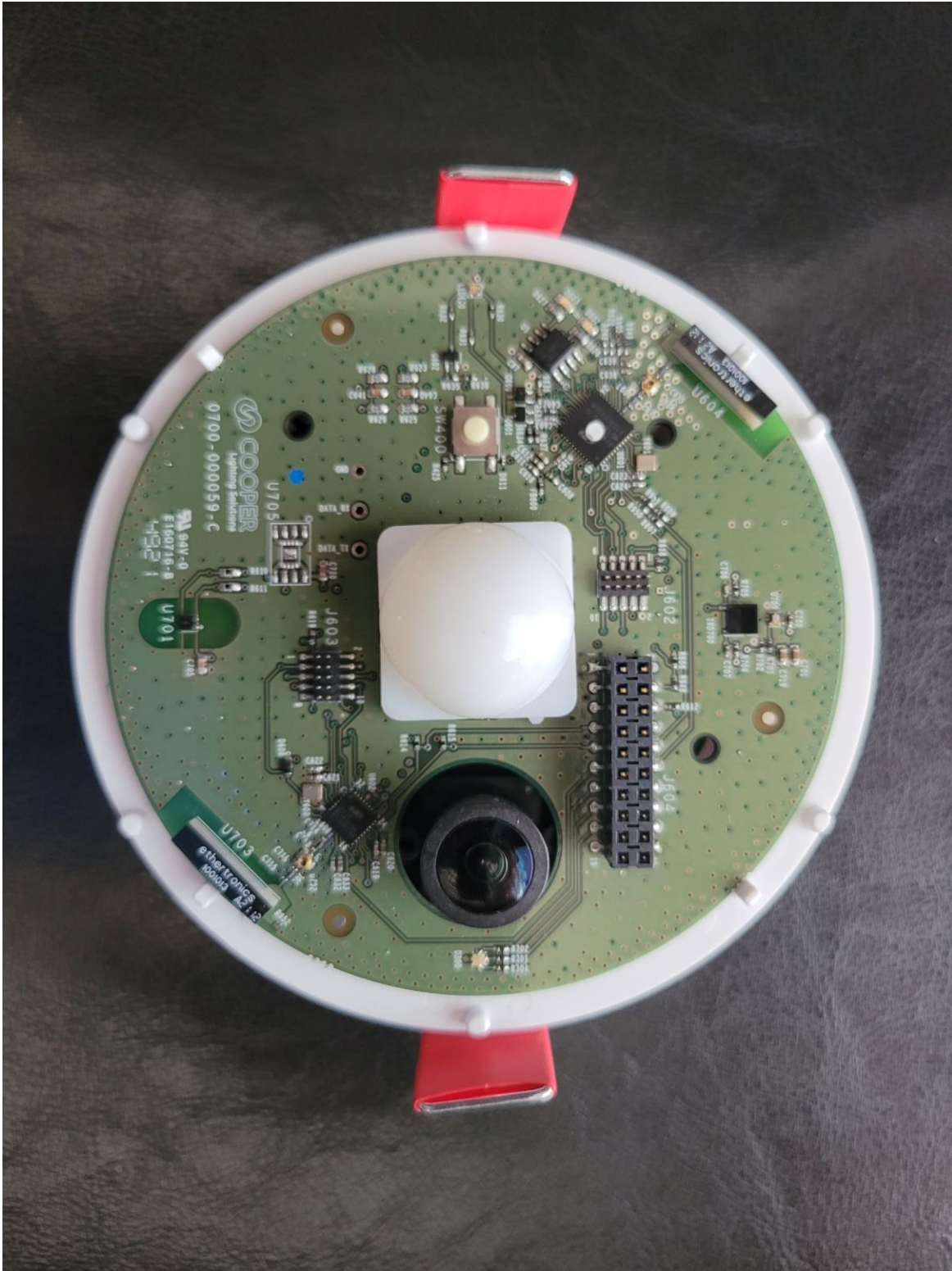
Figure 3: Assembled View
