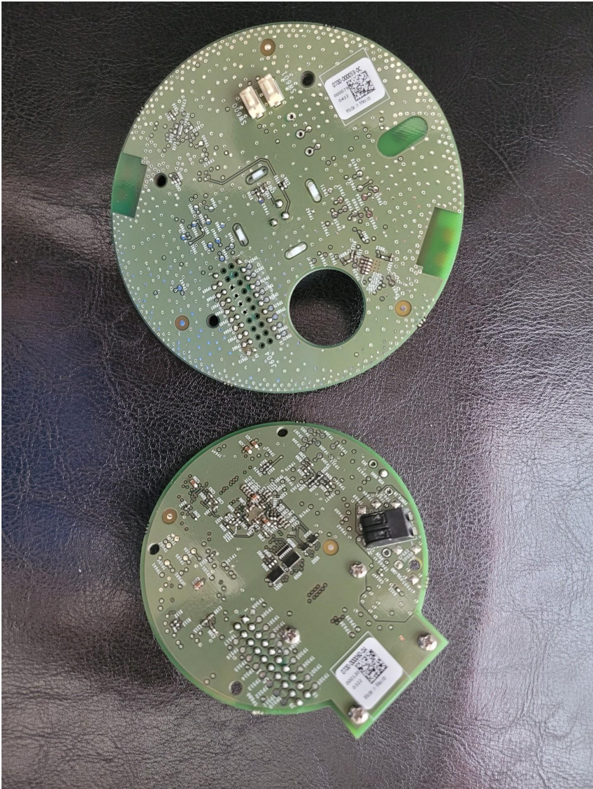
Figure 2: Bottom View
