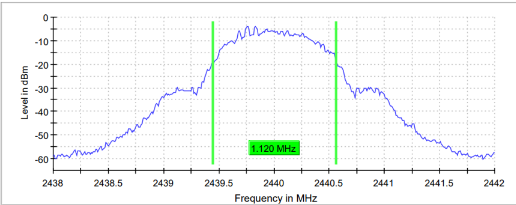
Figure 2.4.6-5: 99% BW - MCH
