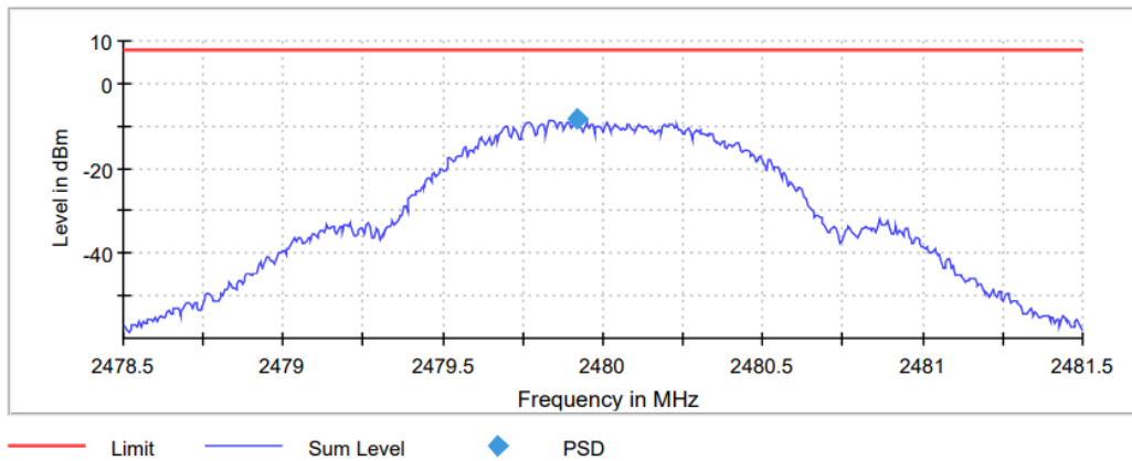
Figure 2.5.6-3: PSD – HCH
