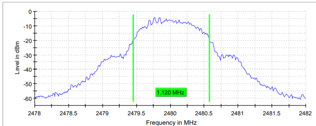
Figure 2.4.6-6: 99% BW - HCH
