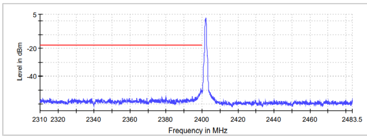
Figure 2.6.6-1: Lower Band-edge
