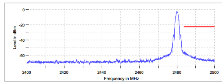
Figure 2.6.6-2: Upper Band-edge
