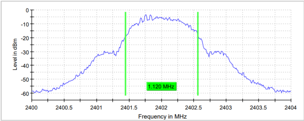
Figure 2.4.6-4: 99% BW - LCH
