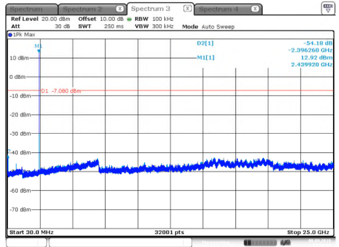
Figure 7.5.1.2-2: MCH – 30MHz–25GHz
