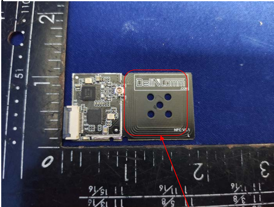
13.56MHz Antenna
