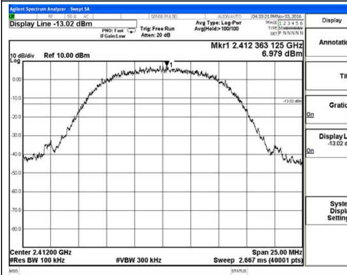
IEEE 802.11b-Low channel Reference
