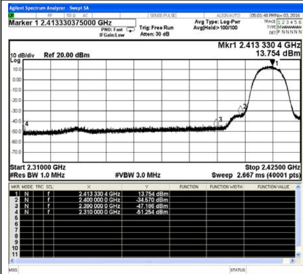
IEEE 802.11b-Low channel(Peak)
