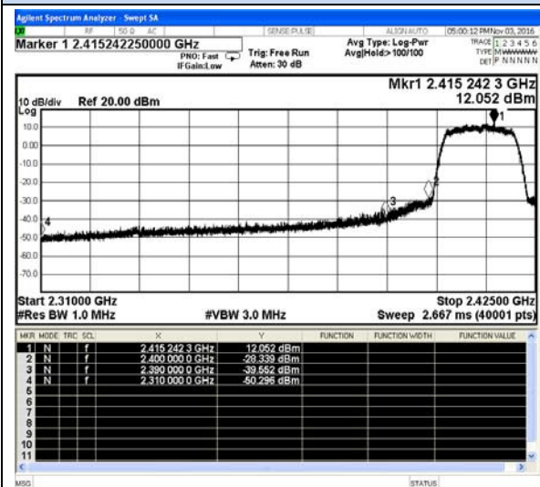
IEEE 802.11g-Low channel(Peak)
