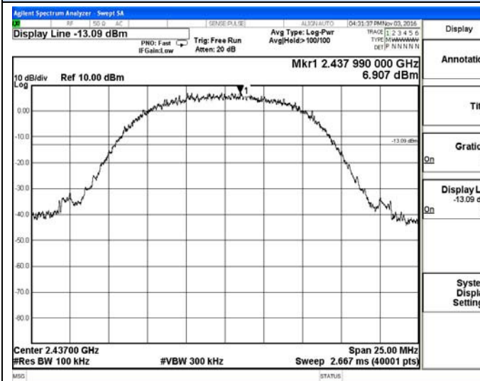
IEEE 802.11b-Middle channel Reference
