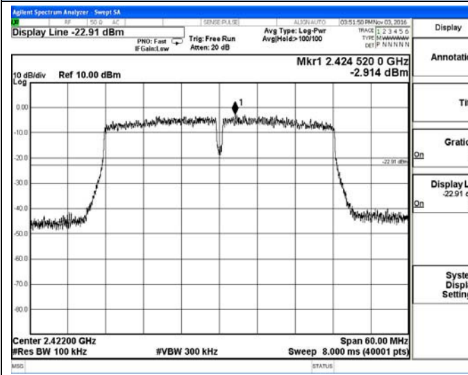
IEEE 802.11n(HT40)-Low channel Reference
