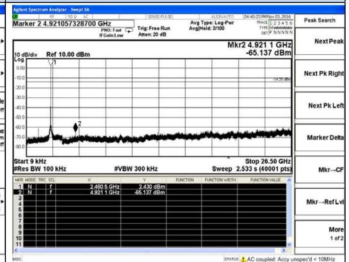
IEEE 802.11b-High channel
