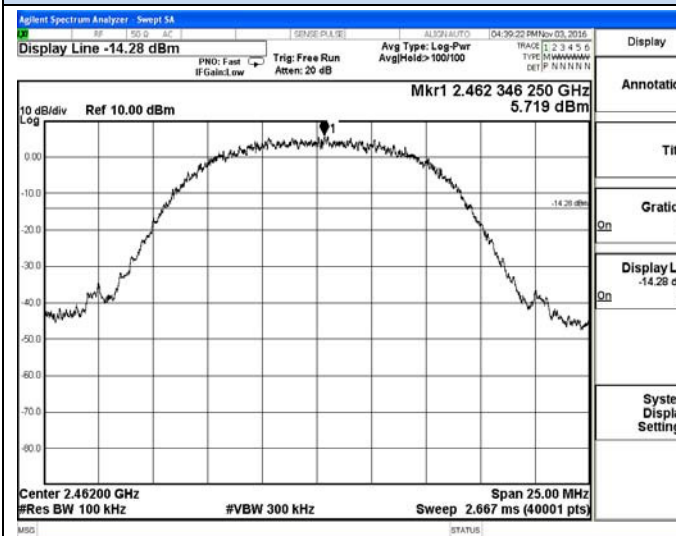
IEEE 802.11b-High channel Reference
