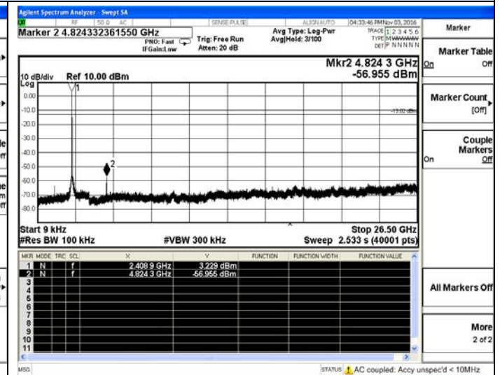
IEEE 802.11b-Low channel
