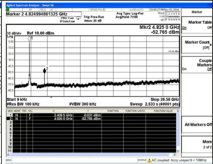
IEEE 802.11n(HT20)-Low channel
