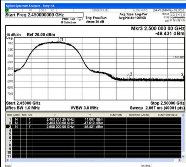
IEEE 802.11b-High channel(Peak)
