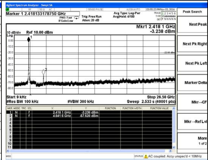
IEEE 802.11n(HT40)-Low channel
