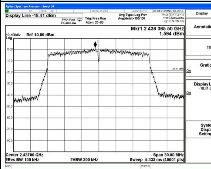
IEEE 802.11n(HT20)-Middle channel Reference
