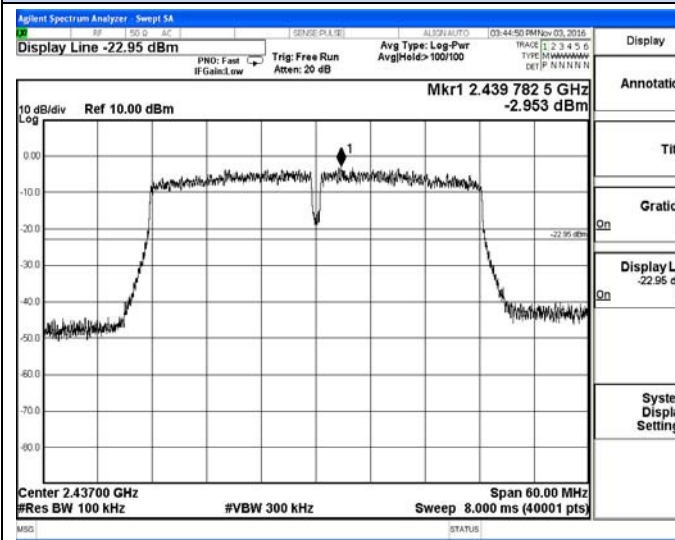
IEEE 802.11n(HT40)-Middle channel Reference
