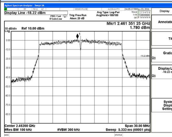
IEEE 802.11n(HT20)-High channel Reference
