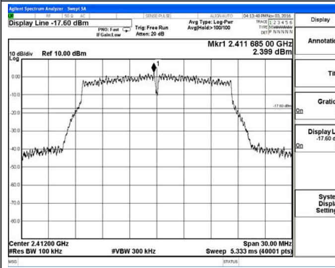
IEEE 802.11g-Low channel Reference
