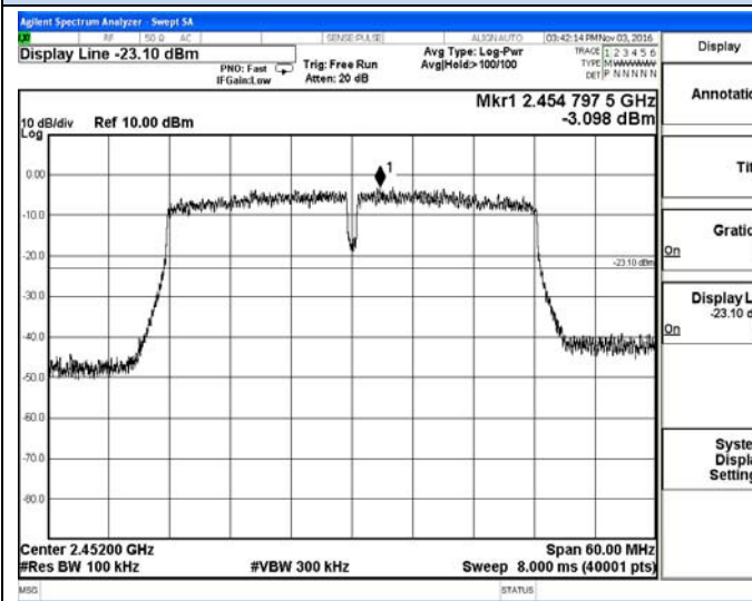
IEEE 802.11n(HT40)-High channel Reference
