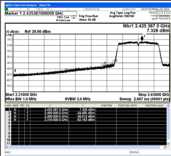
IEEE 802.11n(HT40)-Low channel(Peak)
