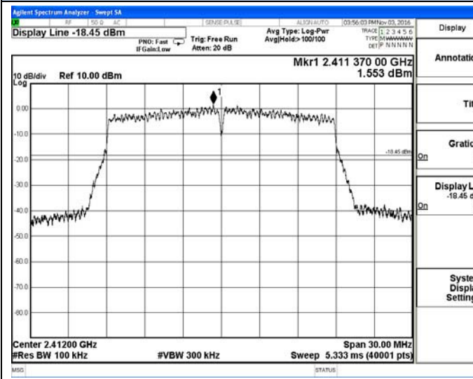
IEEE 802.11n(HT20)-Low channel Reference
