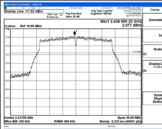
IEEE 802.11g-Middle channel Reference
