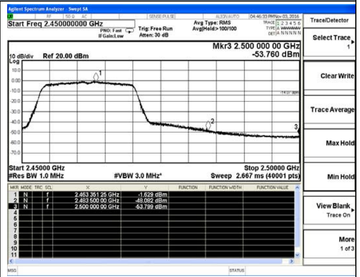
IEEE 802.11g-High channel(Average)
