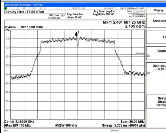
IEEE 802.11g-High channel Reference
