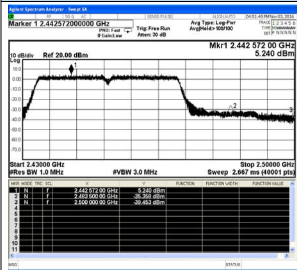
IEEE 802.11n(HT40)-High channel(Peak)
