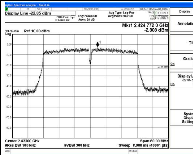
IEEE 802.11n(HT40)-Low channel Reference
