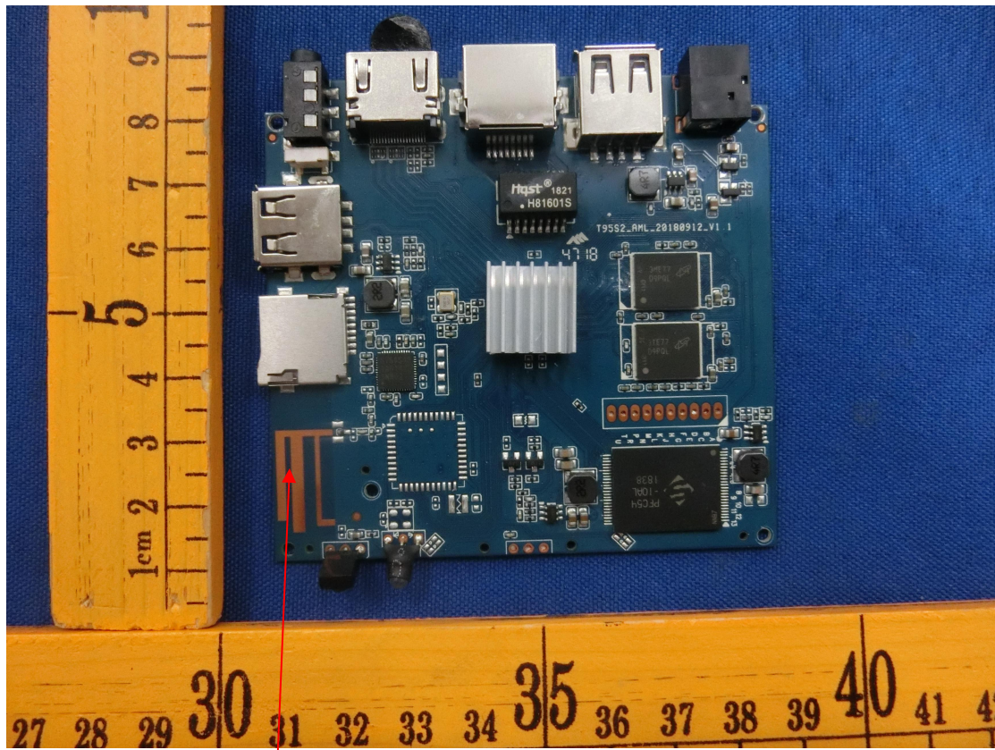
Antenna location
