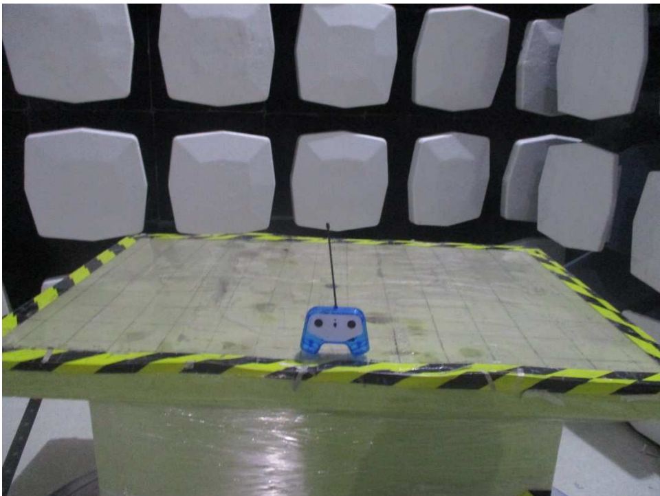
(EUT was placed in the center of the turntable)
