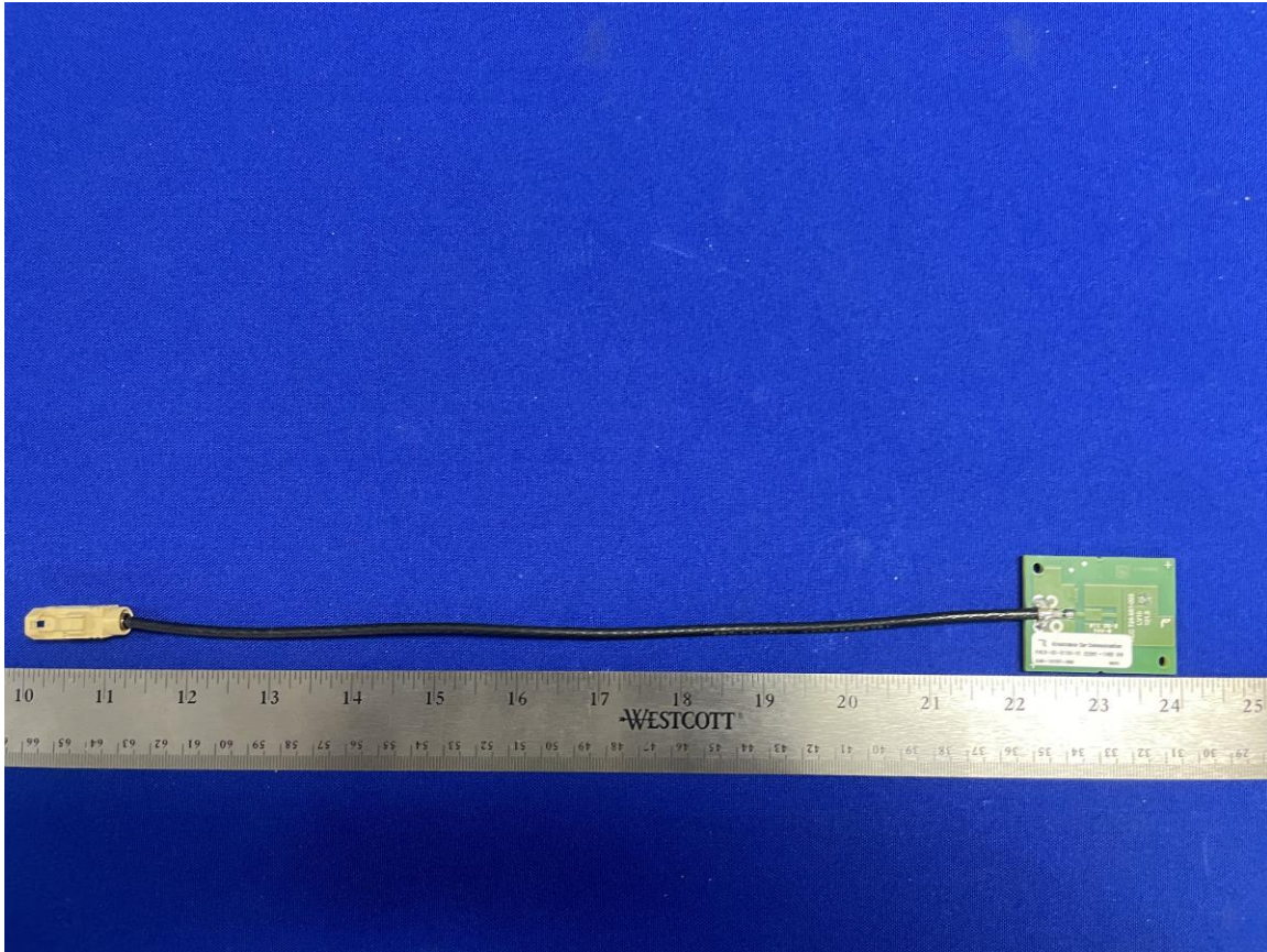
Figure 4: WiFi/ BT Antenna – Top View
