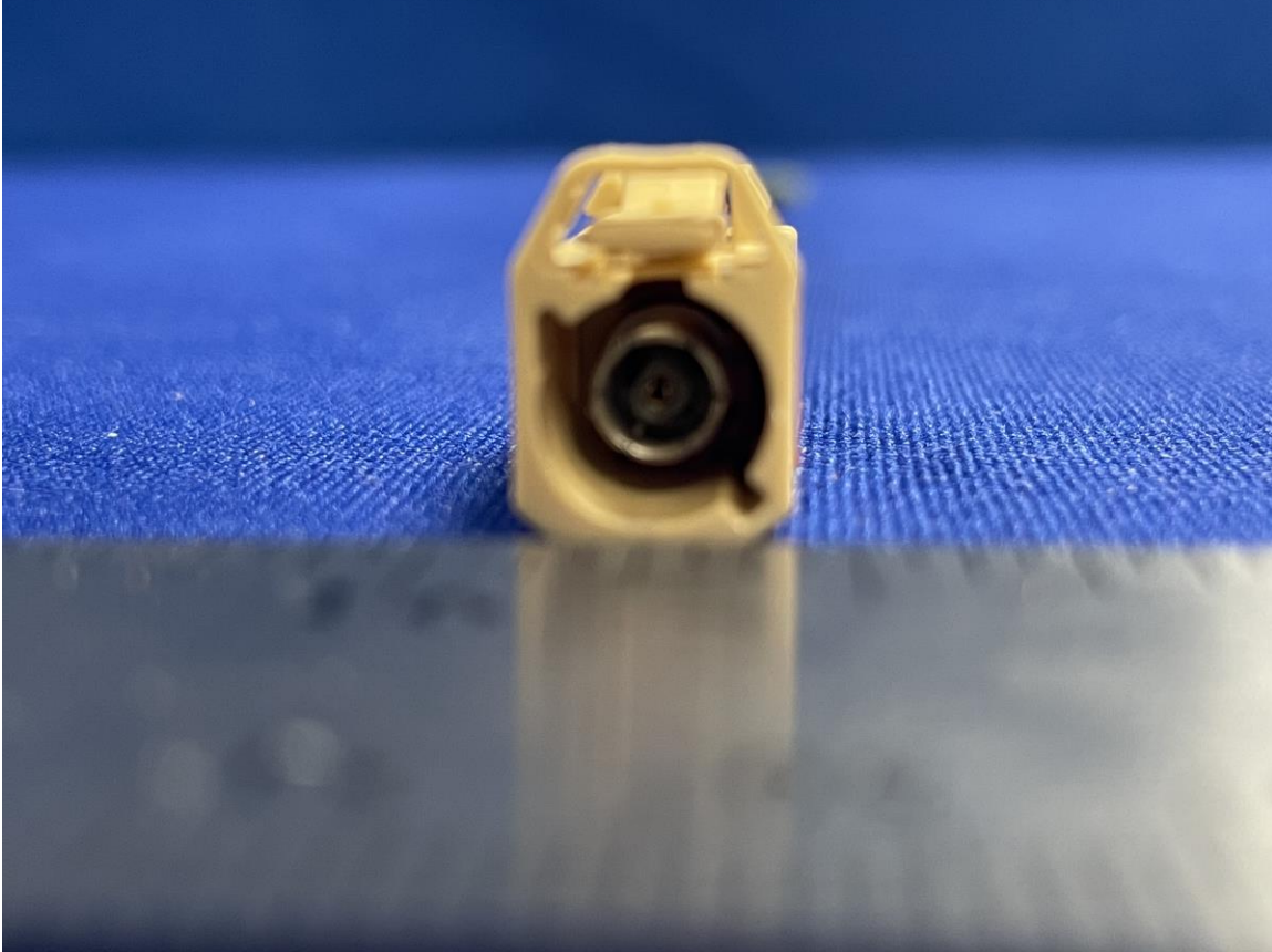
Figure 8: WiFi/ BT Antenna – Connector
