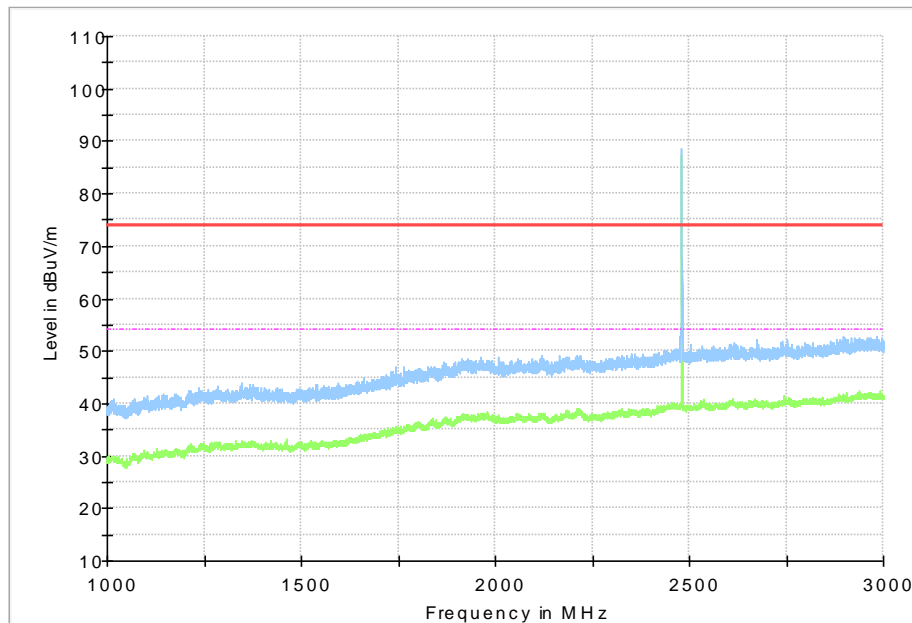
Fig.24 Radiated Spurious Emission (GFSK, Ch39, 1GHz ~3 GHz, Horizontal Direction)
