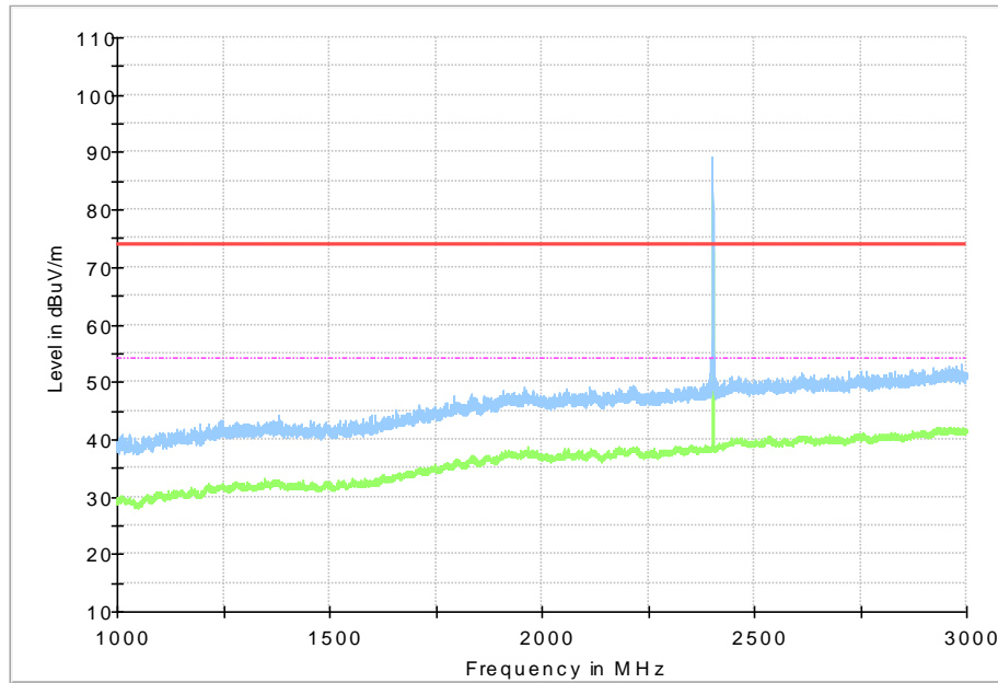
Fig.28 Radiated Spurious Emission (GFSK, Ch0, 1GHz ~3GHz , Vertical Direction)
