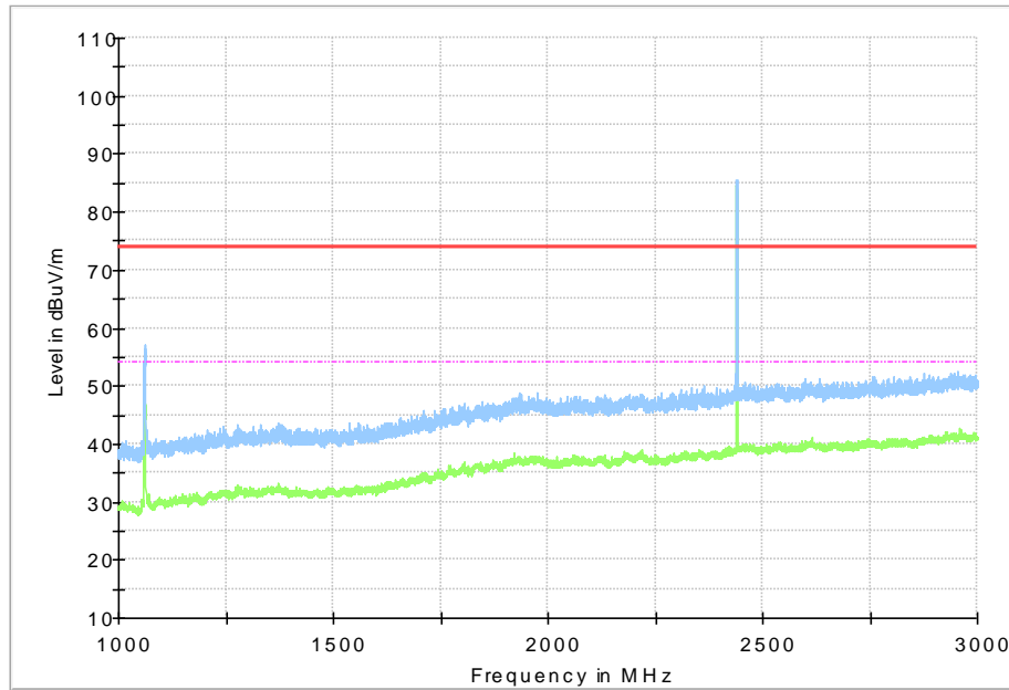
Fig.22 Radiated Spurious Emission (GFSK, Ch19, 1GHz ~3 GHz, Horizontal Direction)
