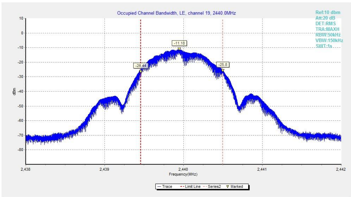
Fig.40 Occupied Bandwidth: GFSK, Channel 19
